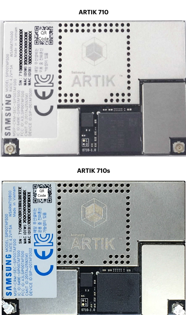
Figure 1. ARTIK™ 710/710s Modules Top View
