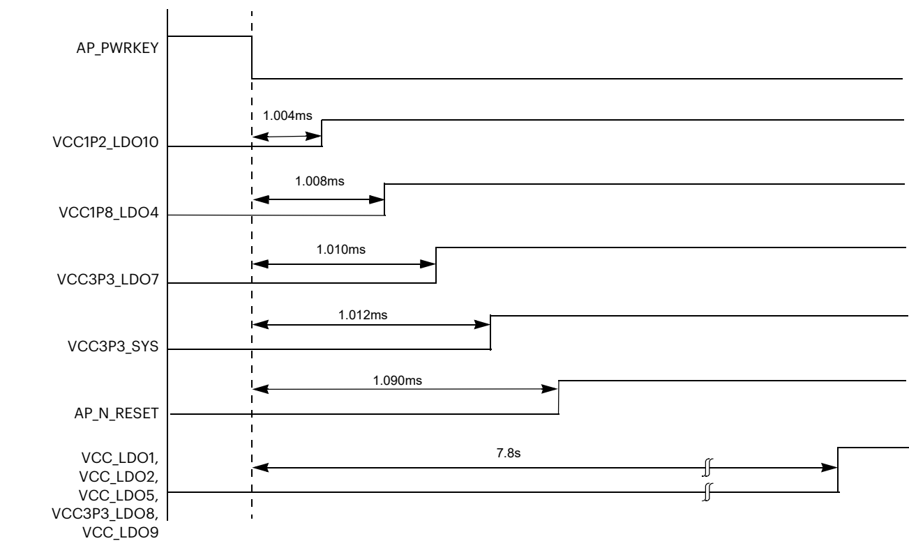
Figure 4. ARTIK 710/710s Module Power-On Sequence (Timing) Diagram
