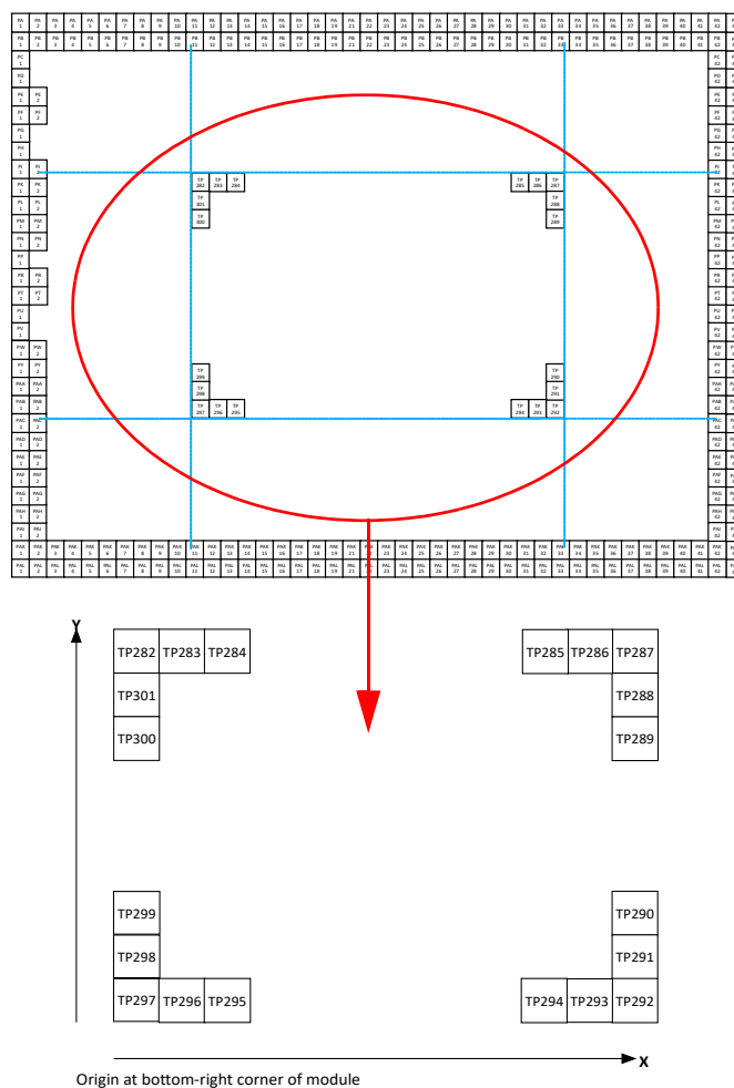
Figure 14. L-Shaped Pad Pins (Top View)
