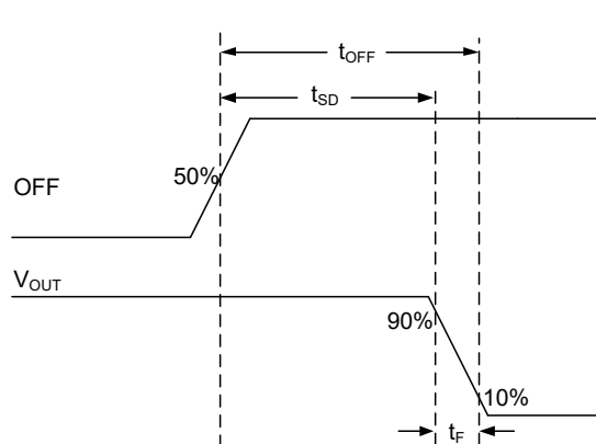
Figure 4. Timing Diagram (OFF vs. VOUT)
