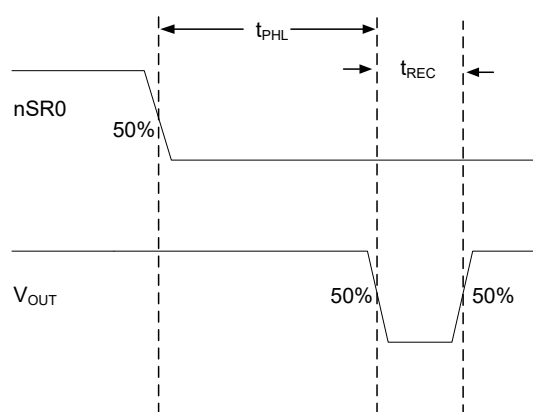
Figure 2. RESET Timing
