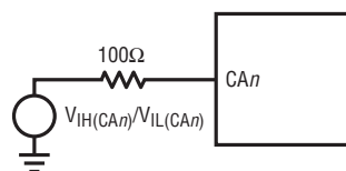
Test Circuit 1
