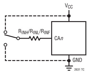
Test Circuit 2
