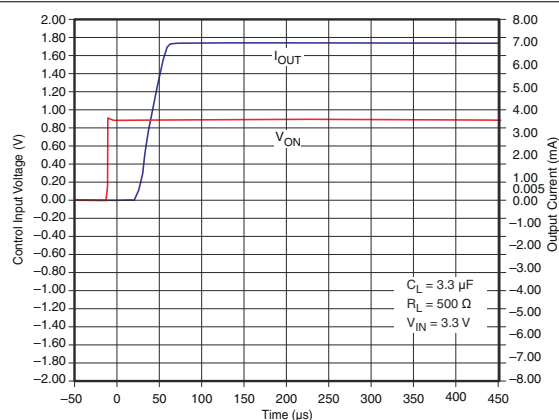
Figure 7-19. t_{ON} Response
