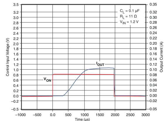
Figure 7-46. t_{ON} Response
