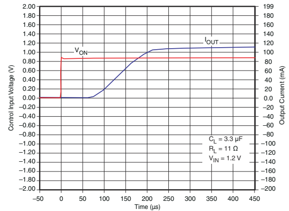
Figure 7-24. t ON Response
