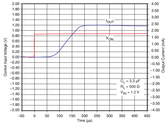
Figure 7-23. t ON Response
