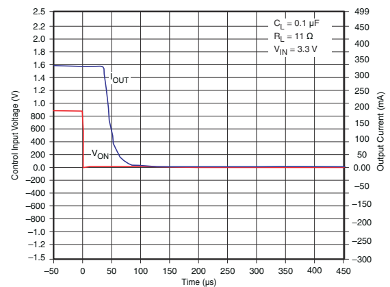
Figure 7-26. t OFF Response
