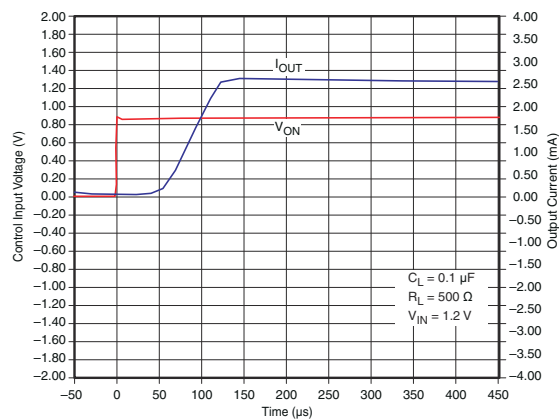
Figure 7-21. t_{ON} Response
