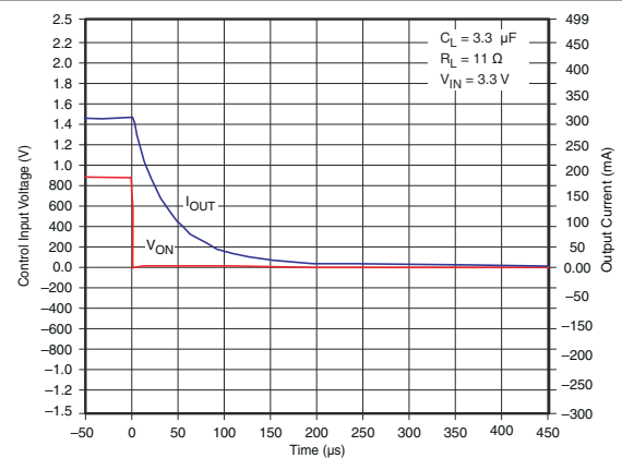
Figure 7-28. t OFF Response
