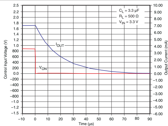
Figure 7-27. t OFF Response
