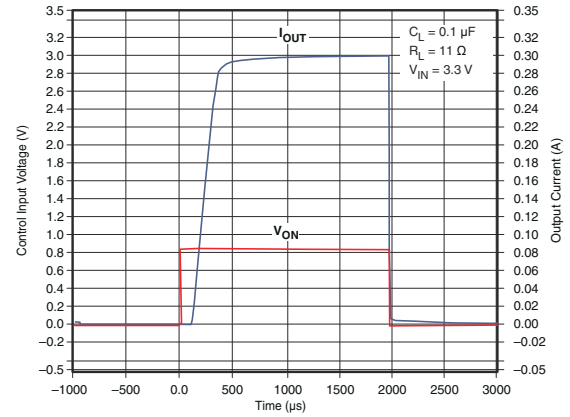
Figure 7-42. t_{ON} Response
