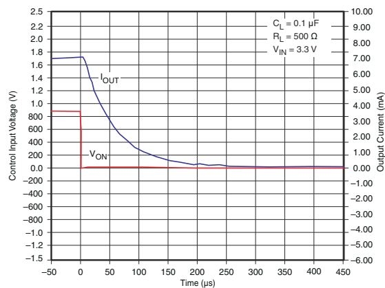
Figure 7-25. t OFF Response
