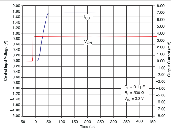
Figure 7-17. t_{ON} Response
