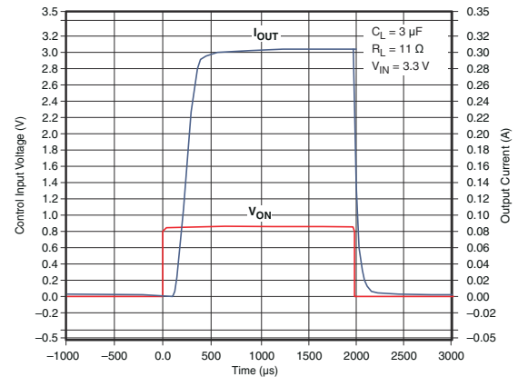
Figure 7-44. t_{ON} Response
