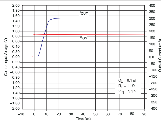
Figure 7-18. t_{ON} Response
