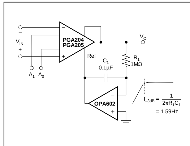
FIGURE 10. AC-Coupled PGIA.
