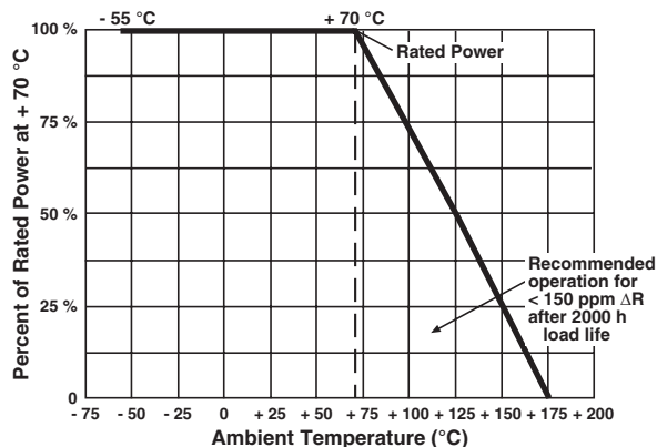
FIGURE 3 - POWER DERATING CURVE 300144, 300145
