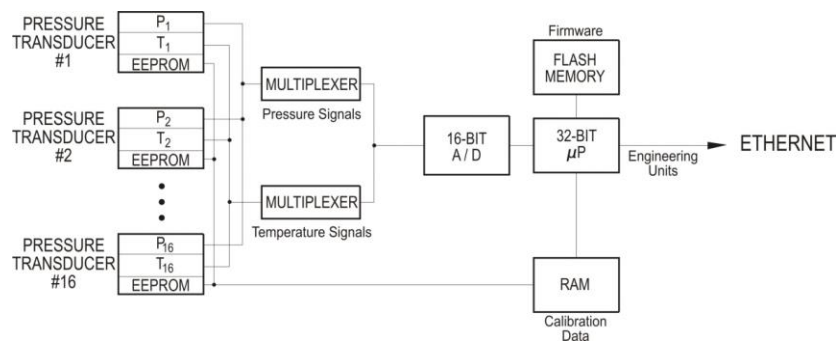
Digital Sensor Temperature Compensation Functional Diagram
