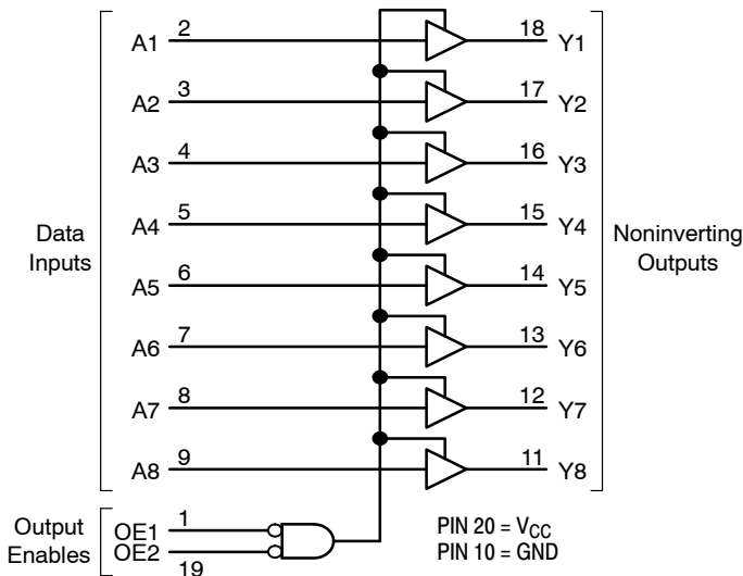
Figure 2. Logic Diagram
