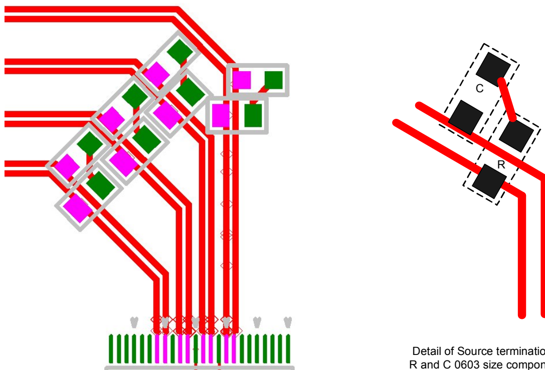
Figure 15. Source Termination Layout Illustration
