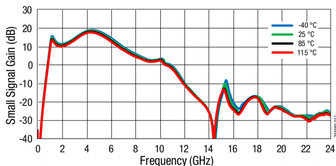
Figure 11. Small Signal Gain (dB) vs Frequency (GHz)
