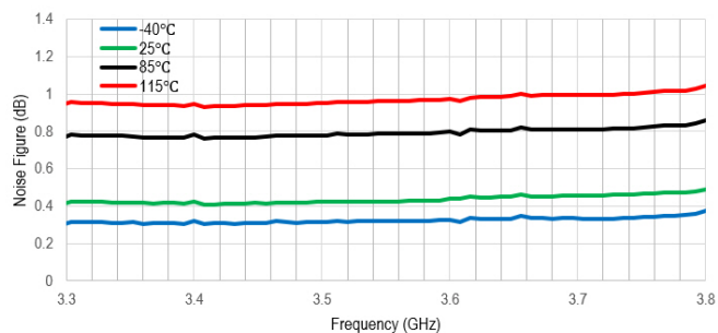
Figure 18. Noise Figure (dB) vs Frequency (GHz)
