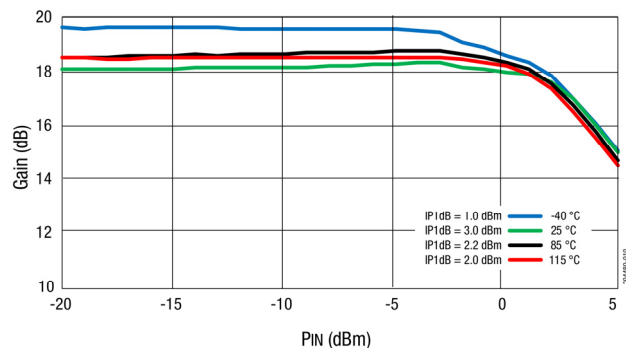
Figure 10. Gain (dB) vs P1dB (dBm)
