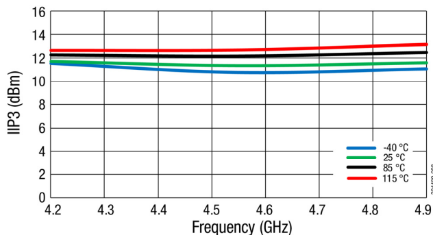
Figure 8. IIP3 (dBm) vs Frequency (GHz)
