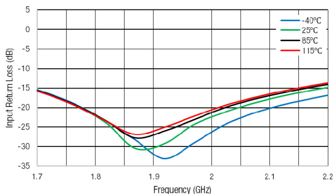
Figure 47. Input Return Loss (dB) vs Frequency
