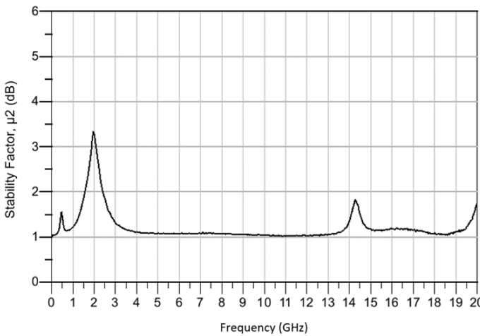
Figure 58. Stability Factor, \mu_2 (dB) vs Frequency (GHz) at -40 °C
