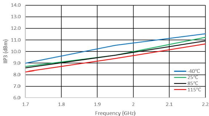
Figure 50. IIP3 (dBm) vs Frequency (GHz)
