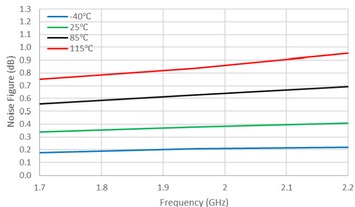
Figure 46. Noise Figure (dB) vs Frequency (GHz)
