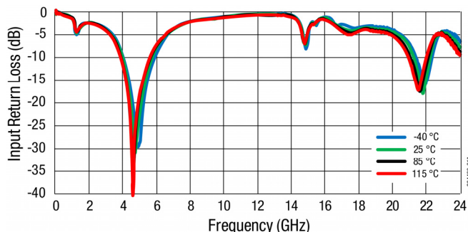
Figure 12. Input Return Loss (dB) vs Frequency (GHz)
