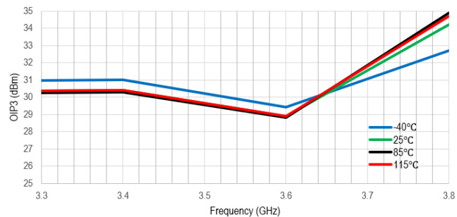
Figure 23. OIP3 (dBm) vs Frequency (GHz)
