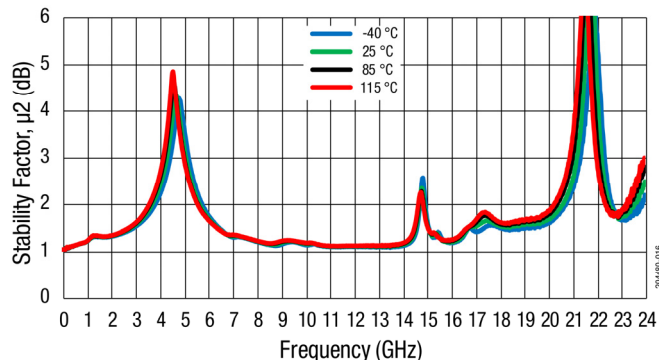
Figure 16. Stability Factor, \mu_2 (dB) vs Frequency (GHz)
