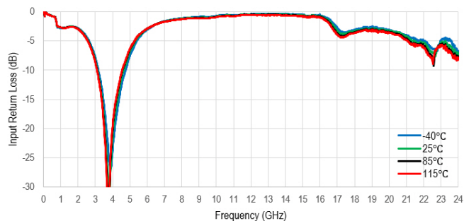
Figure 26. Input Return Loss (dB) vs Frequency (GHz)
