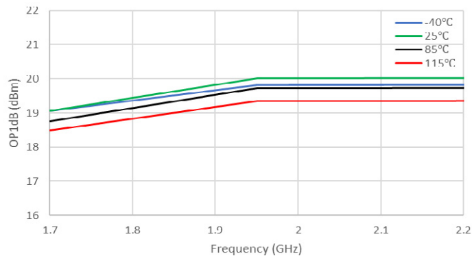
Figure 52. OP1dB (dBm) vs Frequency (GHz)
