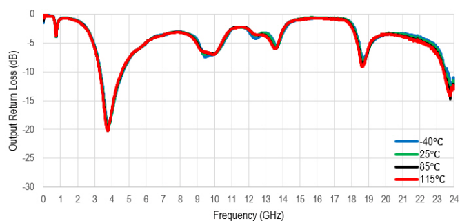
Figure 28. Output Return Loss (dB) vs Frequency (GHz)
