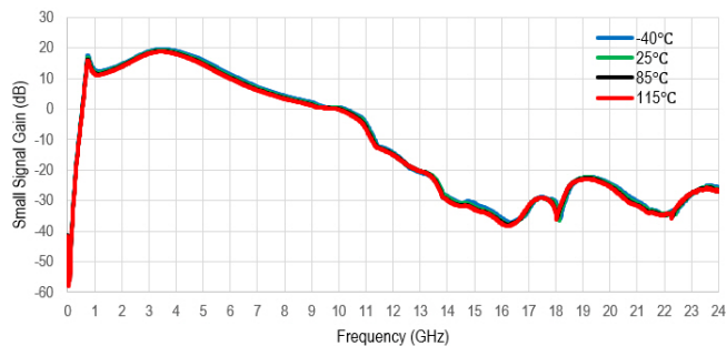
Figure 25. Small Signal Gain (dB) vs Frequency (GHz)
