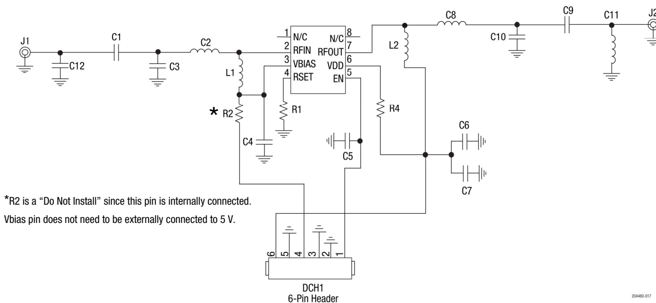
Figure 59. SKY67183-396LF Evaluation Board Schematic
