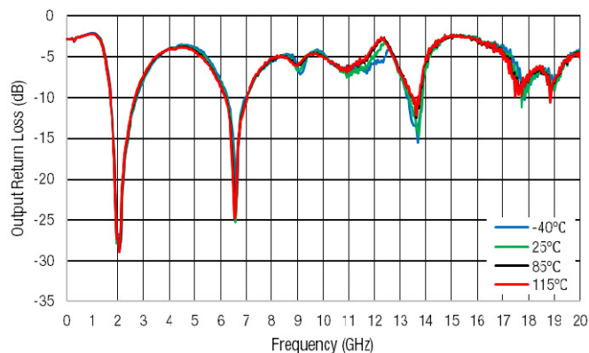
Figure 56. Output Return Loss (dB) vs Frequency (GHz)
