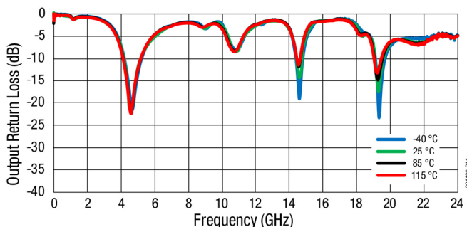
Figure 14. Output Return Loss (dB) vs Frequency (GHz)
