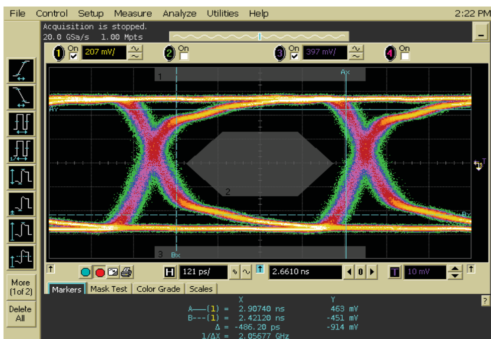
Figure 4: 8bit deep color DVI/HDMI TX eye tested with 20 meter. 24 AWG HDMI cable. Setting: Optimized equalization, 0dB output pre-emphasis and de-emphasis, and Swing 500mV.
