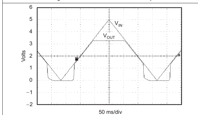
Figure 21. TPS73233 Turnon Response
