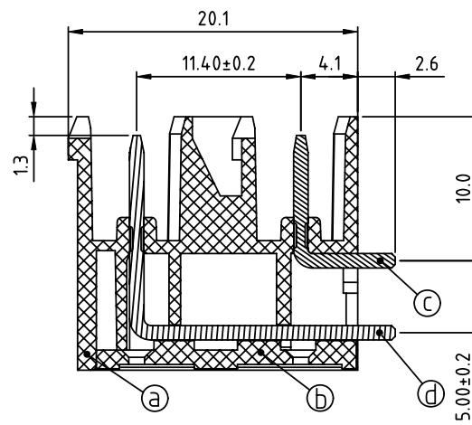
SECTION P-P
