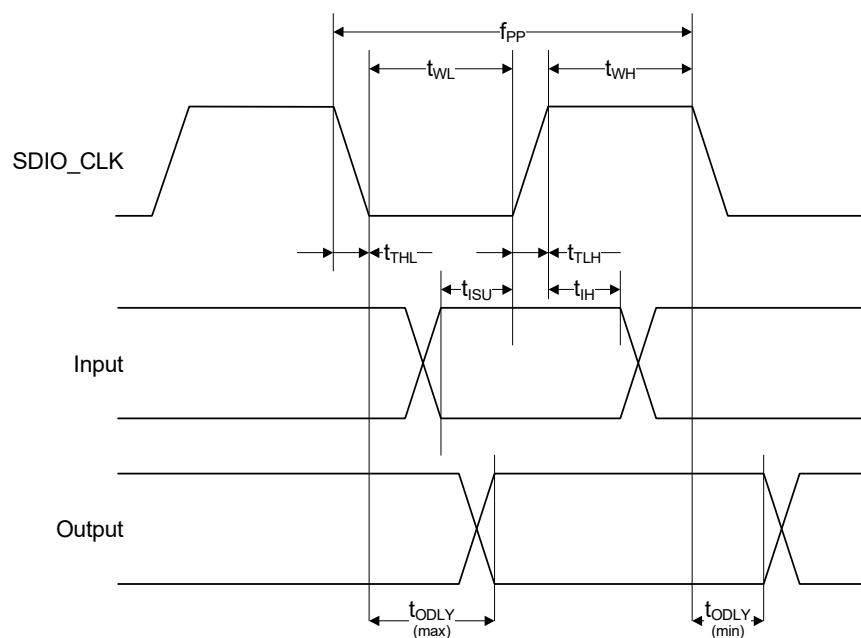
Figure 35. SDIO Bus Timing (Default Mode)
