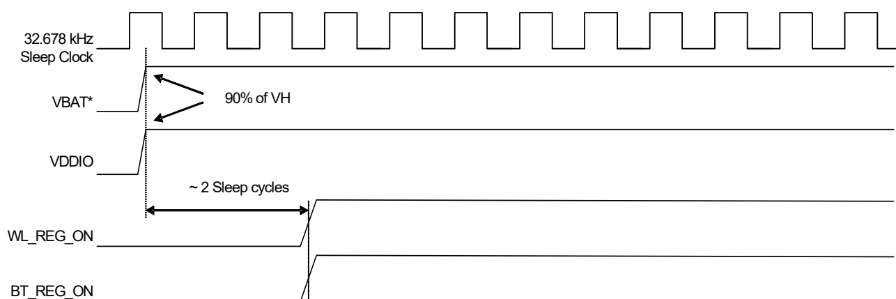
Figure 44. WLAN = ON, Bluetooth = ON
