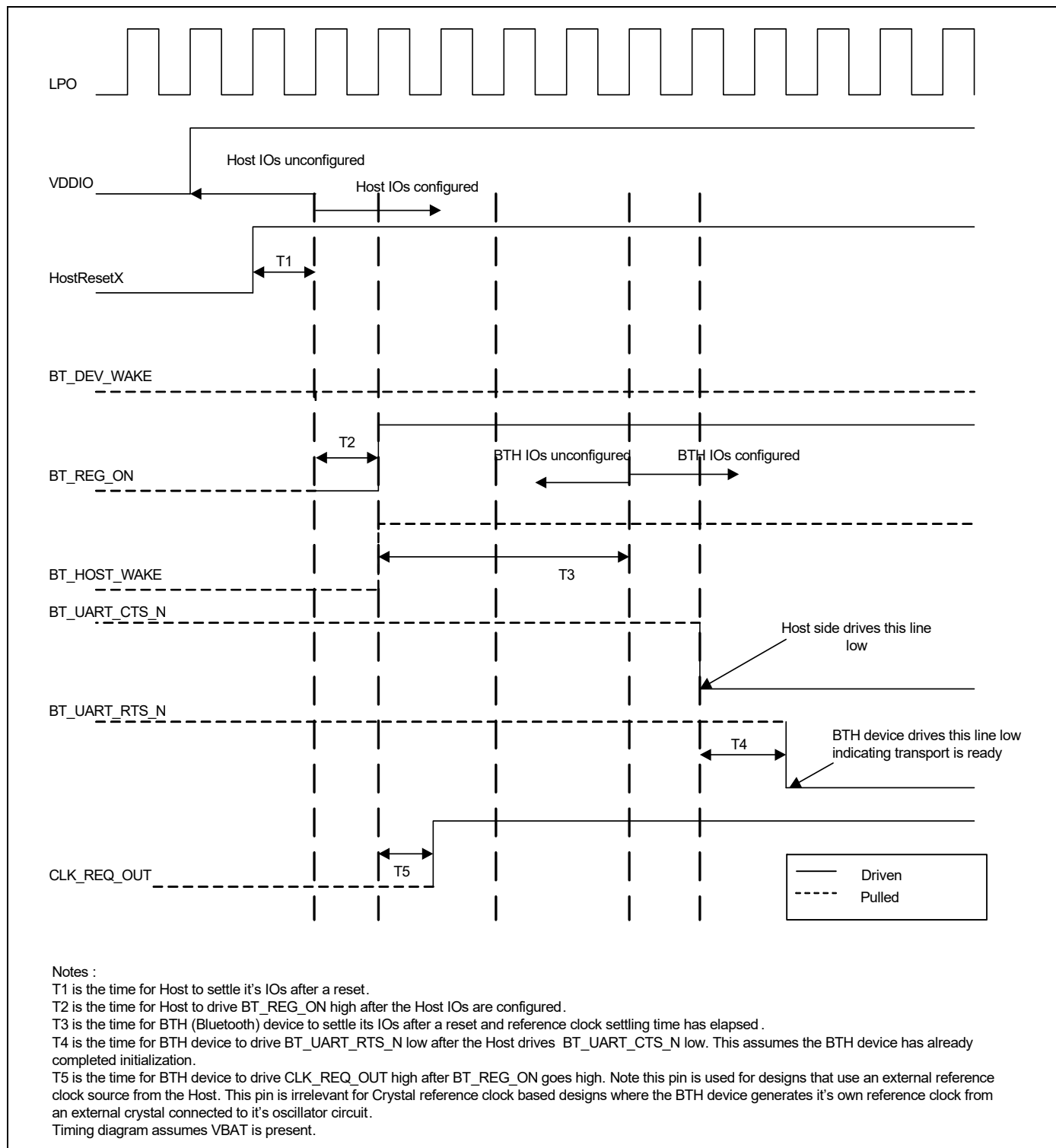
Figure 7. Startup Signaling Sequence Prior to Software Download
