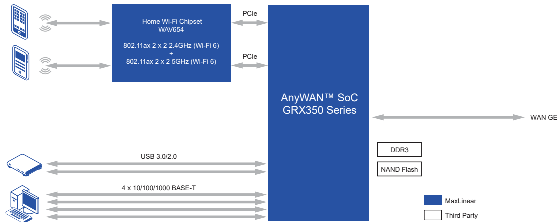
AX3000 Ethernet Router
