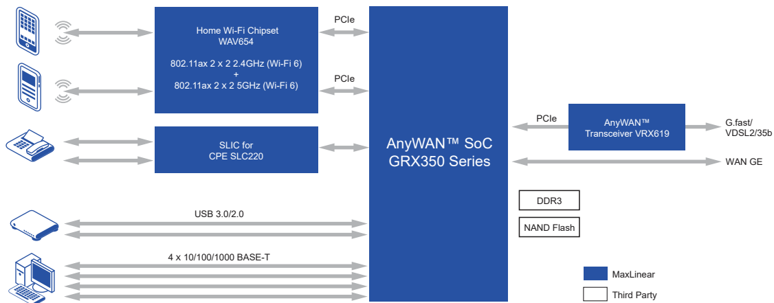
AX3000 G.fast or DSL Gateway
