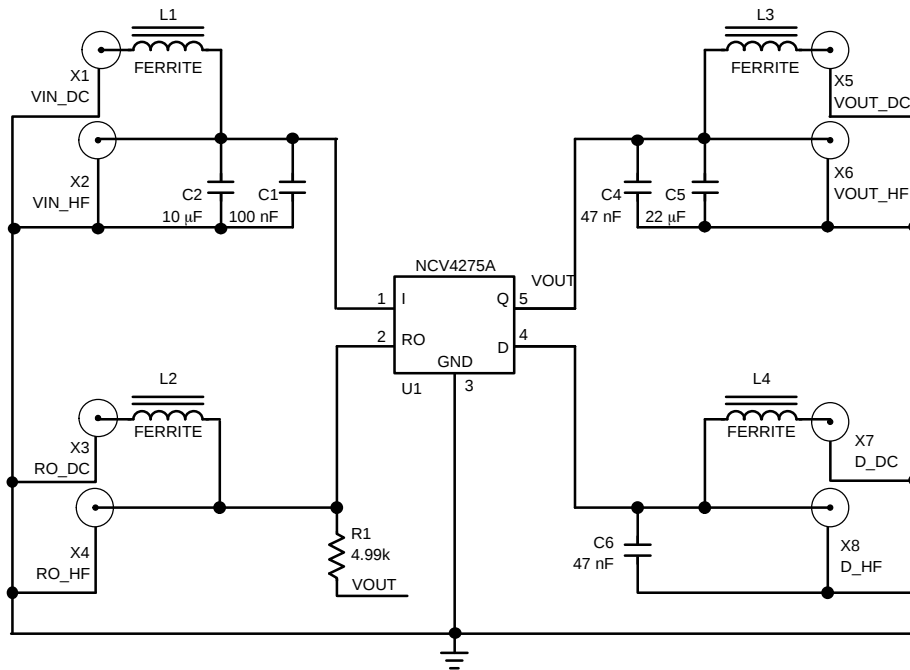
Figure 34. Test Circuit
