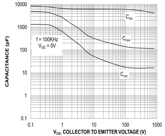
Figure 27. Capacitance Charge
