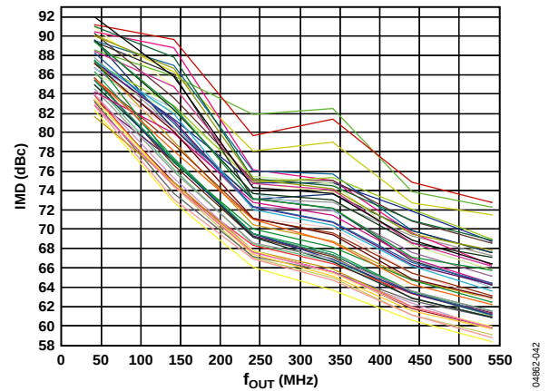
Figure 44. AD9736 IMD vs. f_{OUT} over 50 Parts, 25°C, 1.2 GSPS
