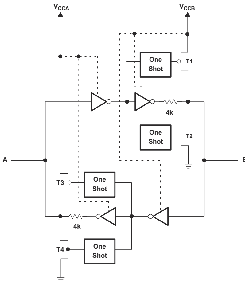
Figure 8-1. Architecture of TXB0104 Device I/O Cell
