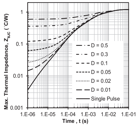
Figure 6: Maximum Transient Thermal Impedance
