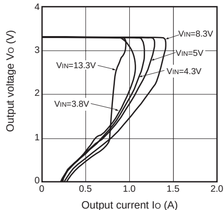
Fig.4 Overcurrent Protection Characteristics (PQ030RDA1SZH)
