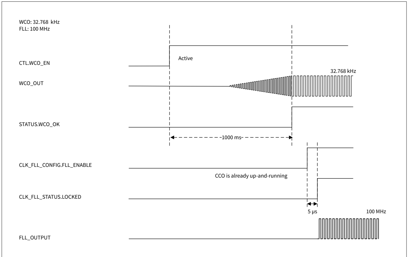
Figure 39 WCO to FLL Diagram
