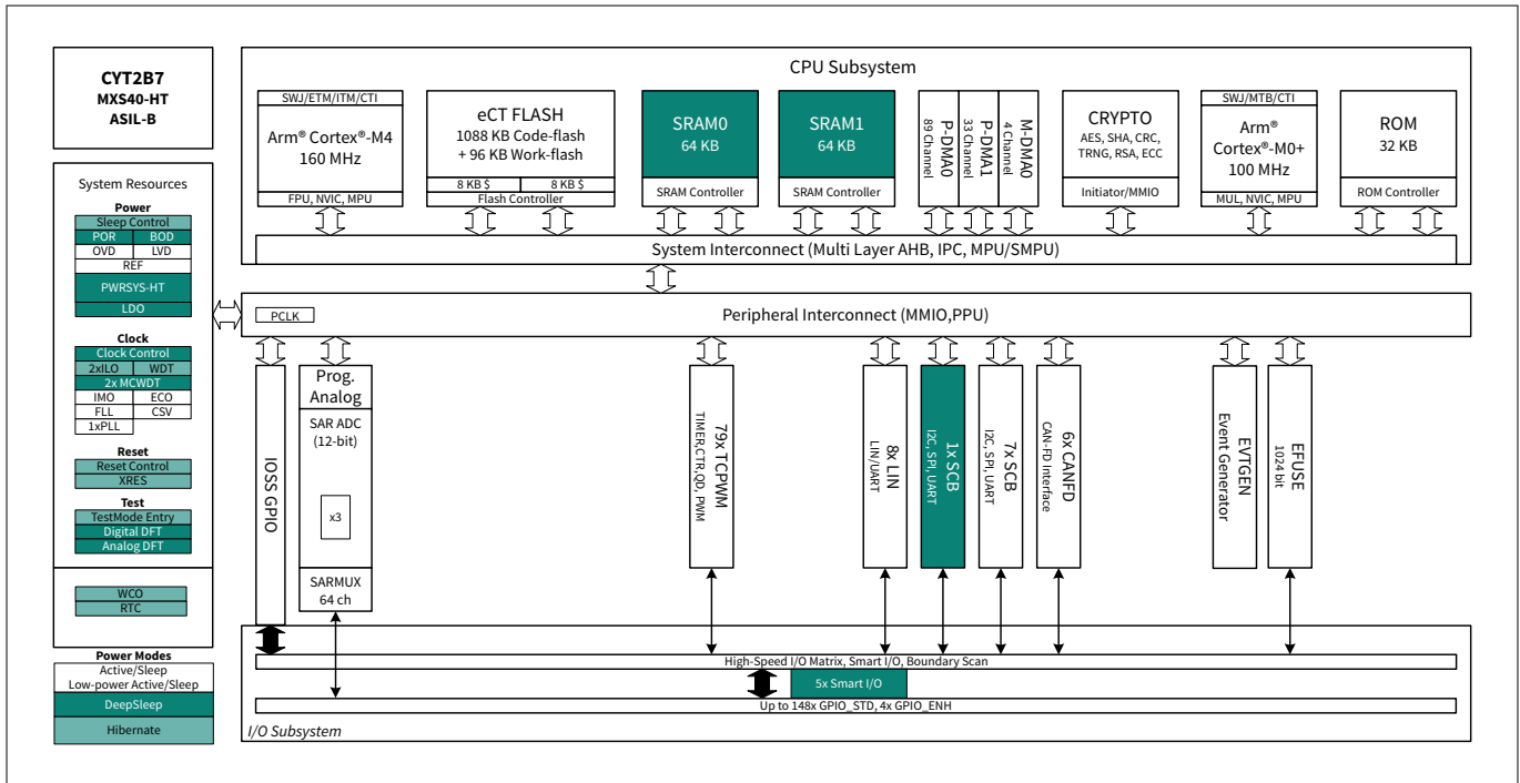
Figure 1 Block diagram
