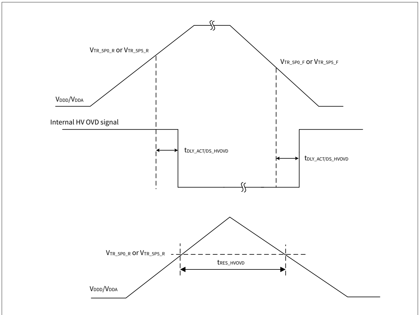
Figure 32 High-voltage OVD specifications
