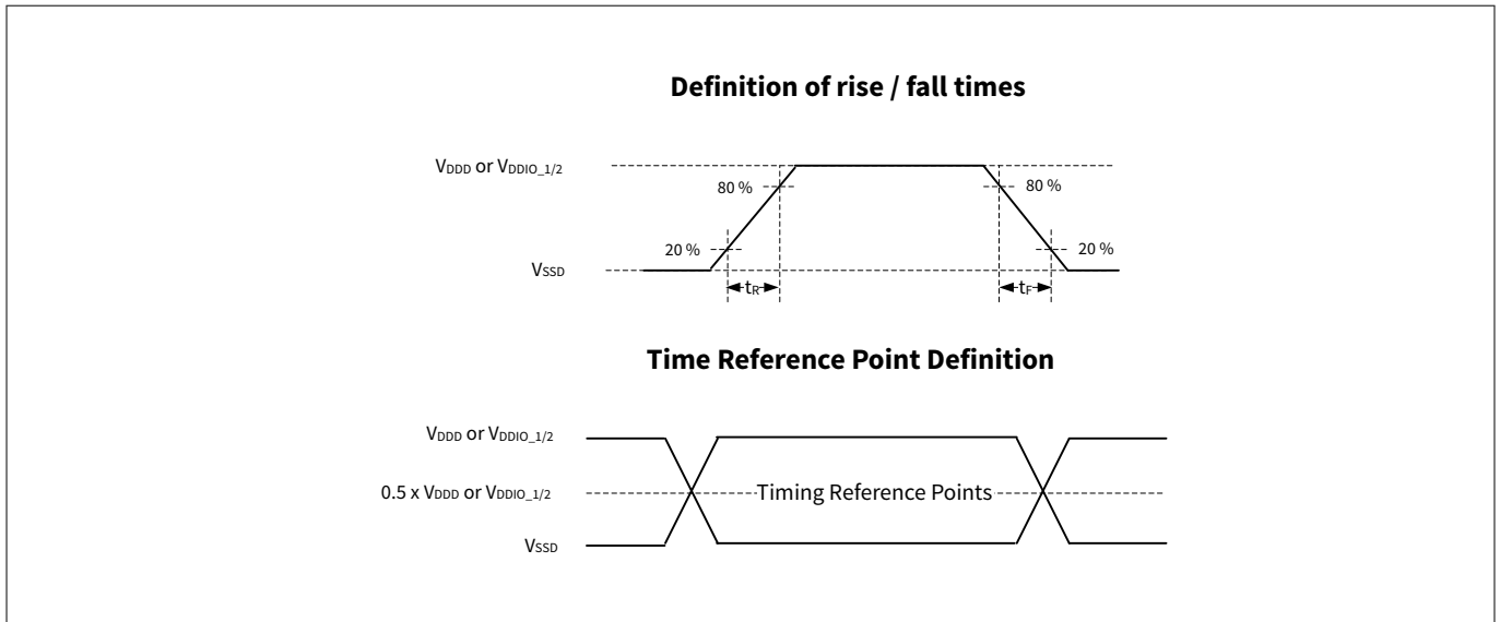
Figure 21 AC timings specifications
