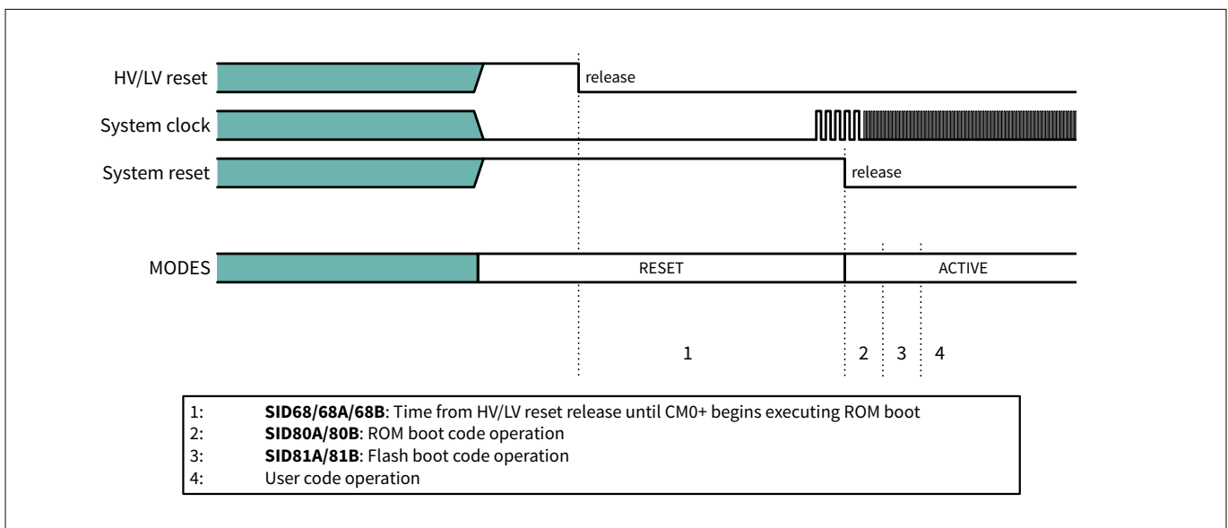
Figure 17 Reset sequence
