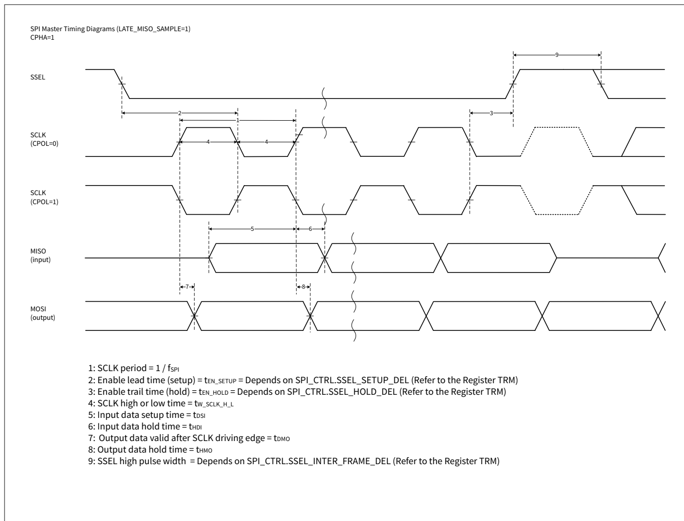
Figure 25 SPI master timing diagrams with HIGH clock phase
