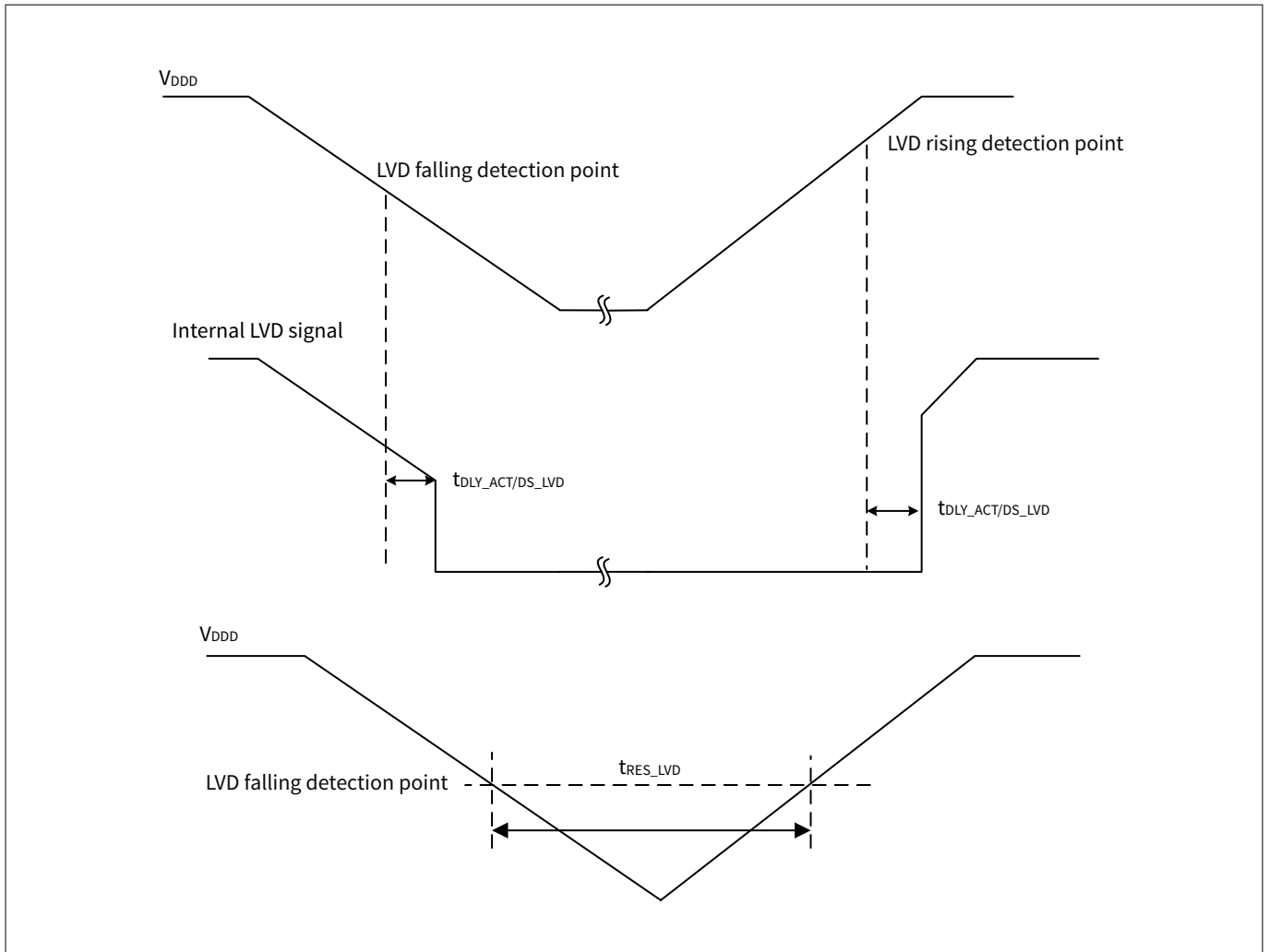
Figure 34 LVD specifications
