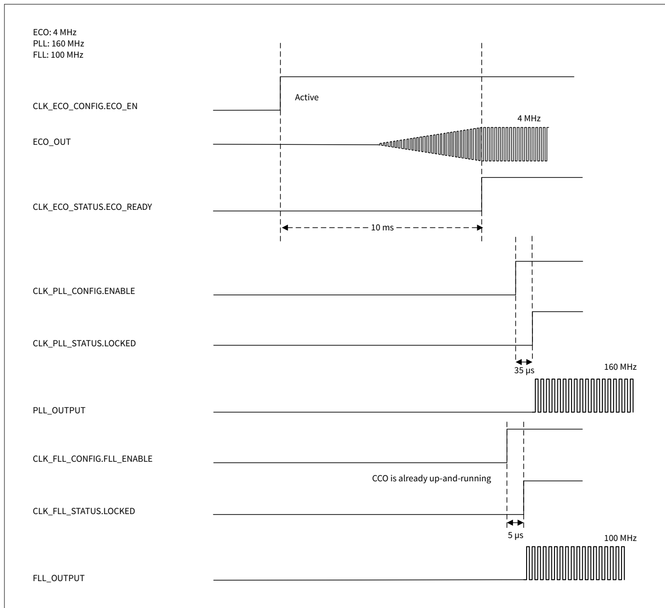
Figure 38 ECO to PLL or FLL diagram
