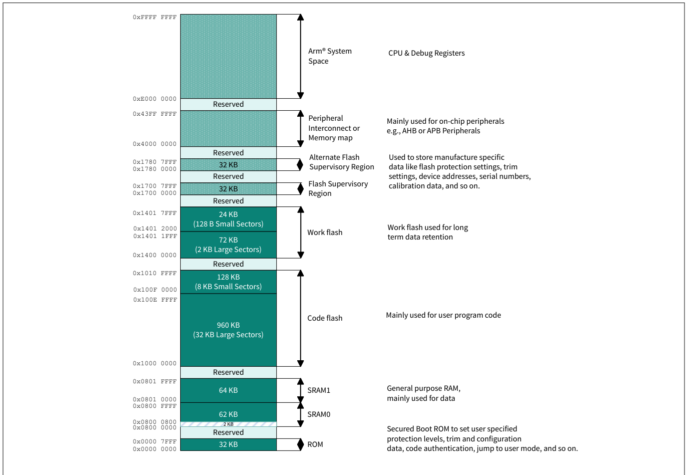
Figure 2 CYT2B7 address map 12), 13)
