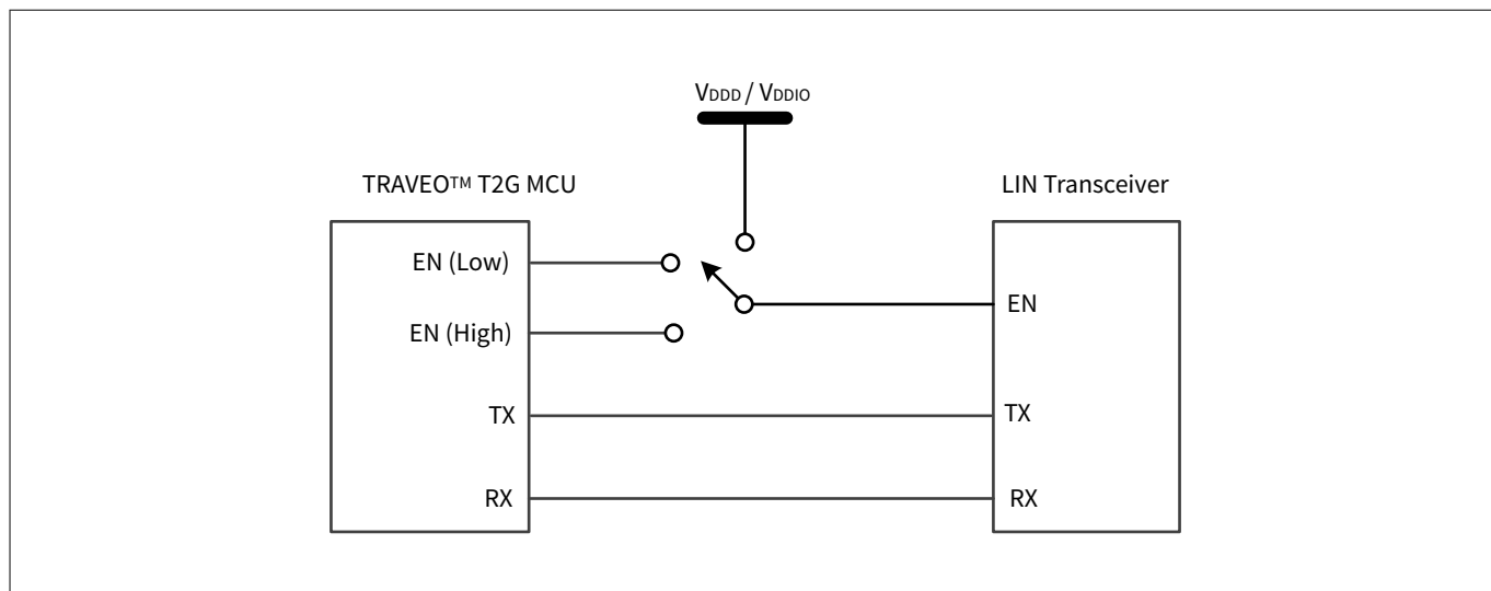
Figure 47 MCU to LIN transceiver connections
