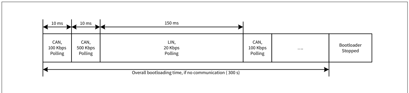
Figure 45 Bootloading sequence
