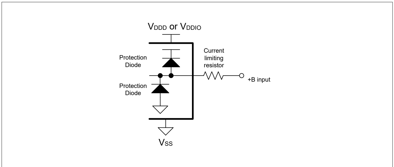
Figure 15 Example of a recommended circuit 16)
