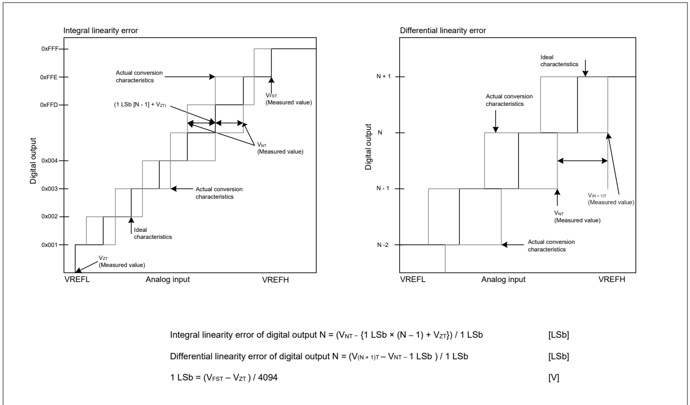
Figure 19 Integral and differential linearity errors
