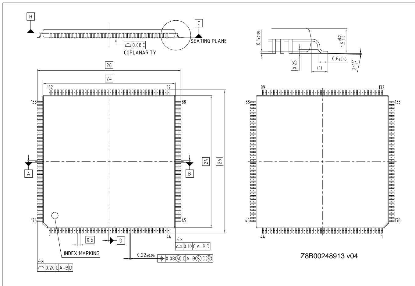
Figure 43 80-LQFP package outline (PG-LQFP-80)
