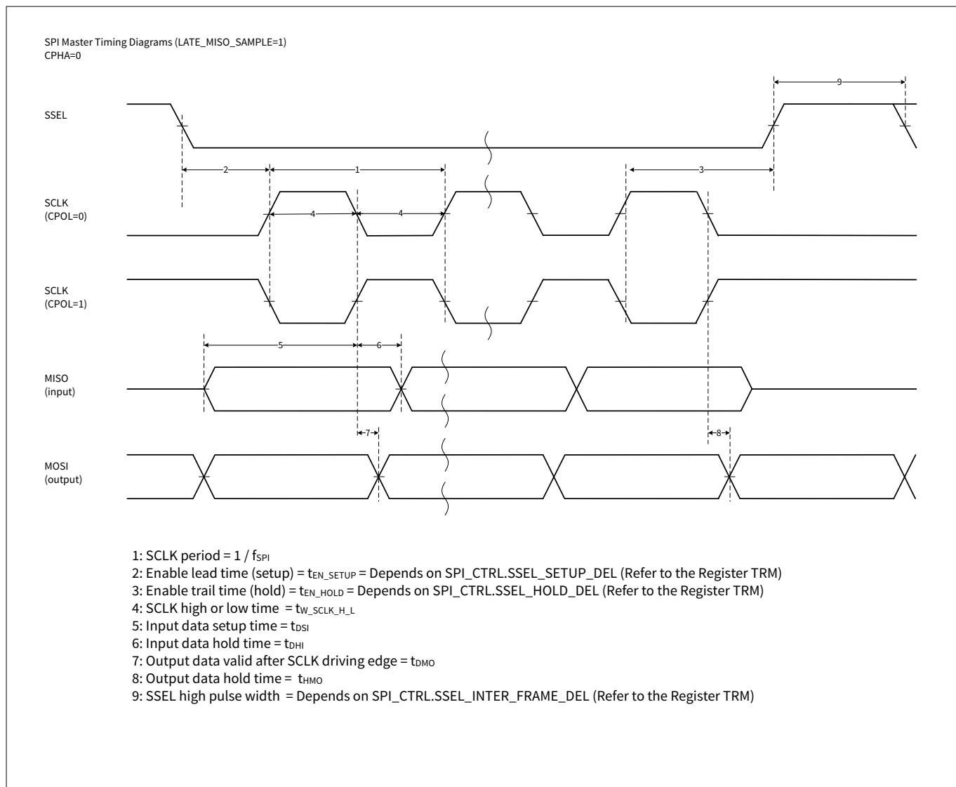
Figure 24 SPI master timing diagrams with LOW clock phase
