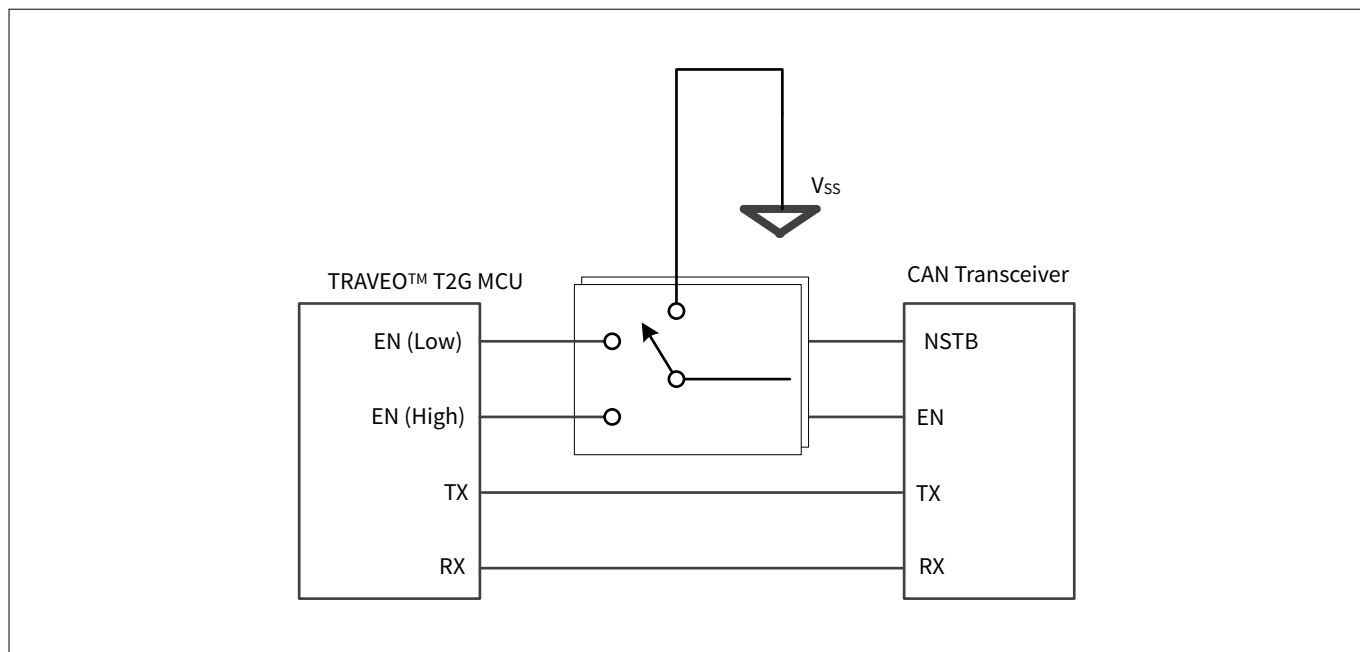
Figure 46 MCU to CAN transceiver connections
