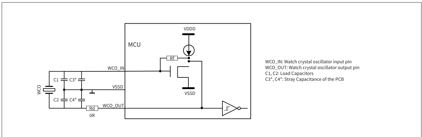
Figure 37 WCO connection scheme 18)
