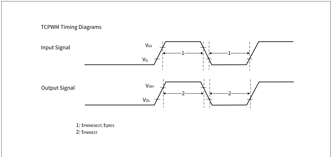
Figure 22 TCPWM timing diagrams
