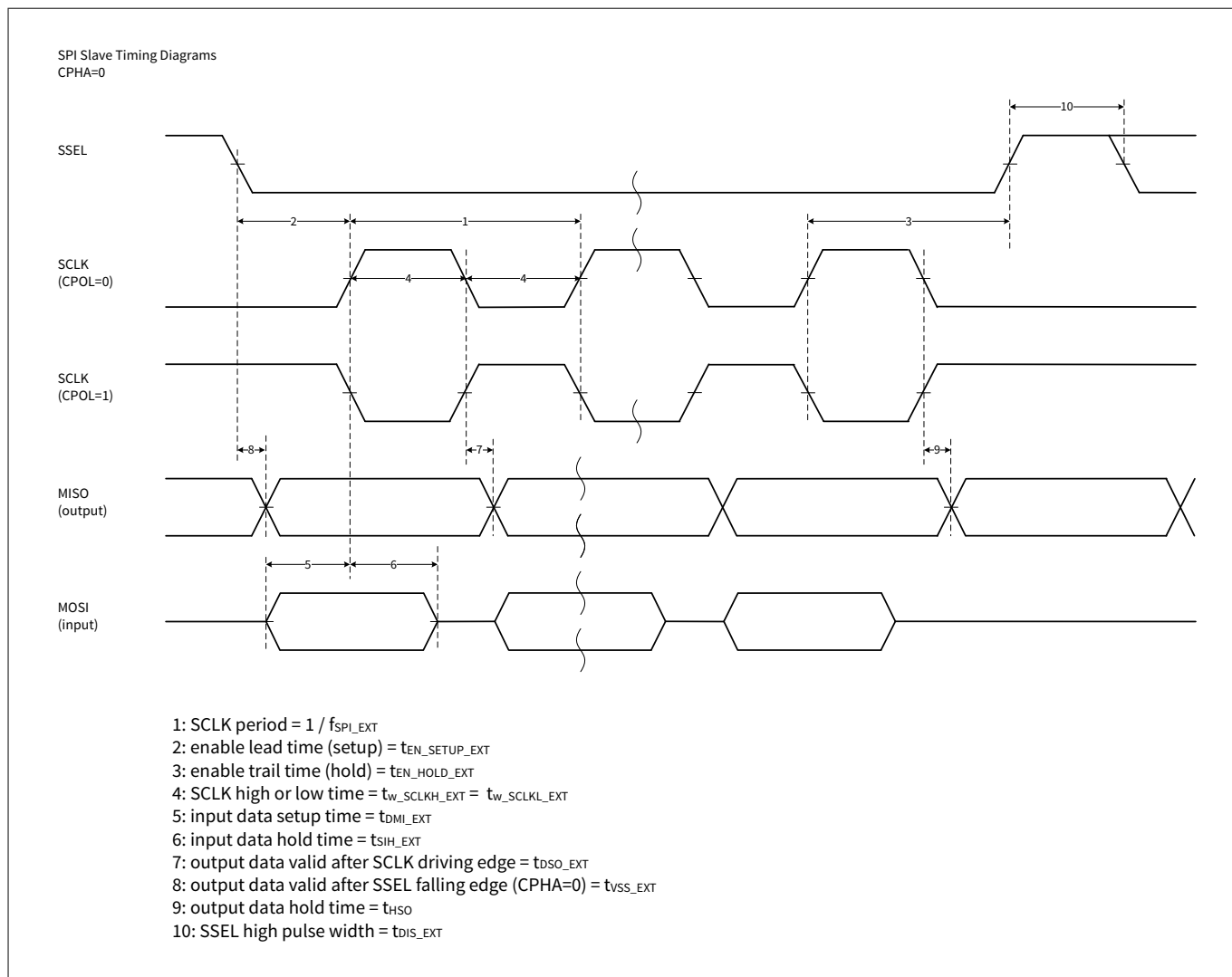
Figure 26 SPI slave timing diagrams with LOW clock phase
