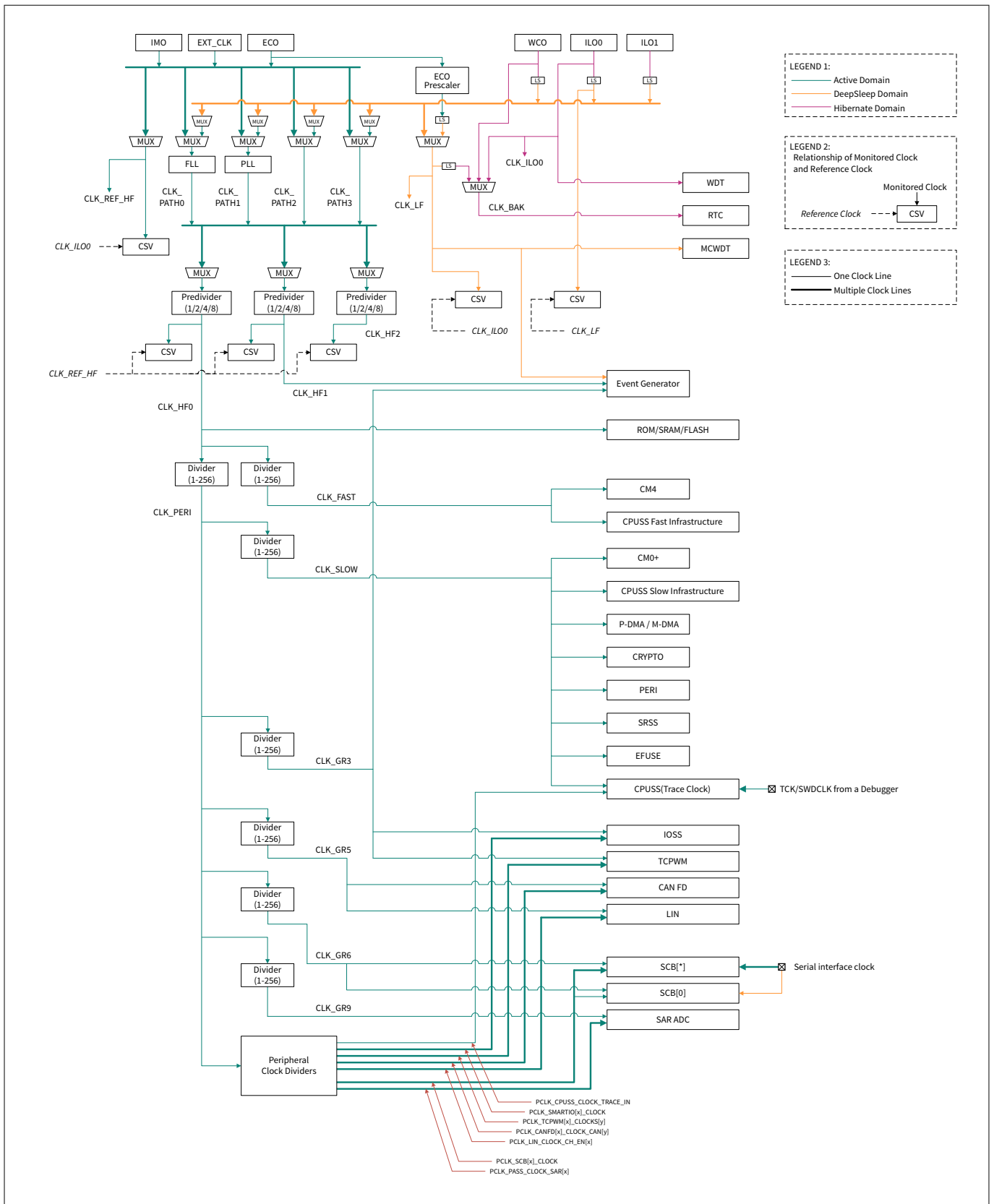
Figure 3 CYT2B7 clock diagram
