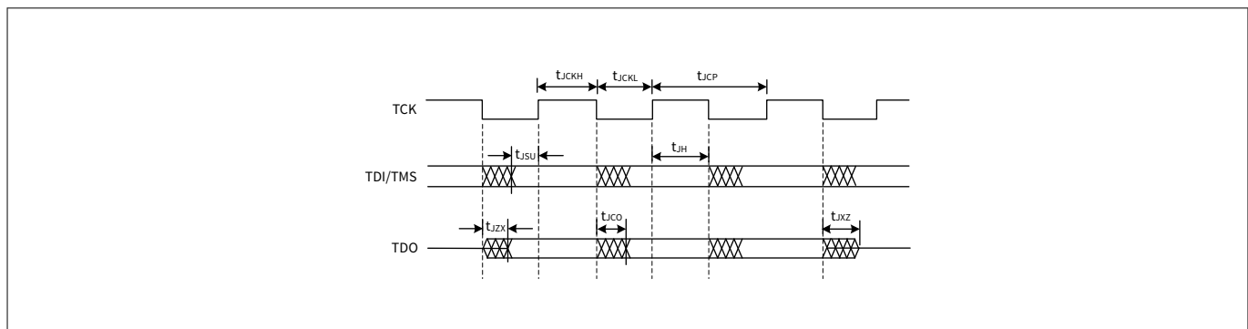
Figure 35 JTAG timing diagram
