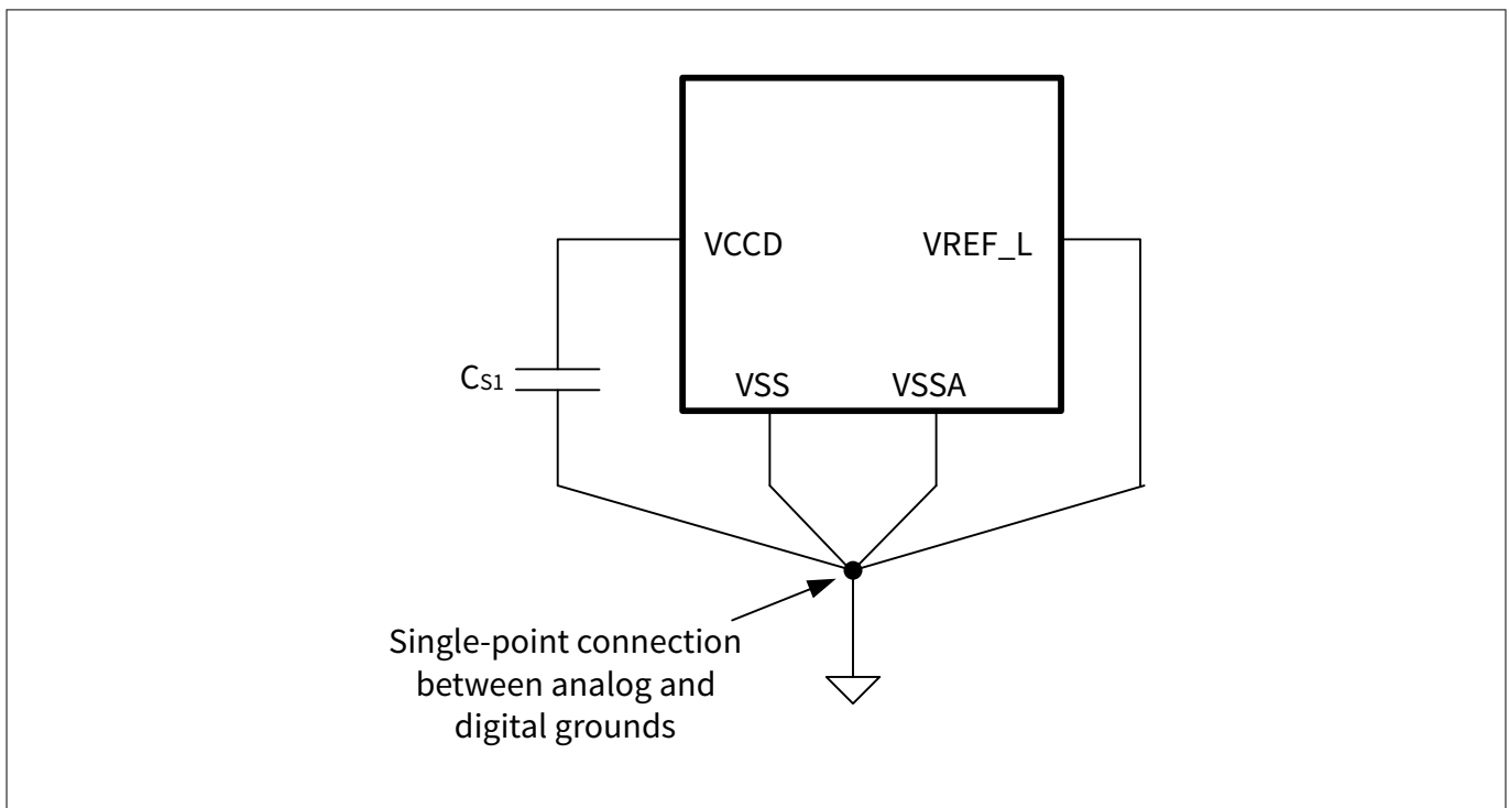
Figure 16 Smoothing capacitor
