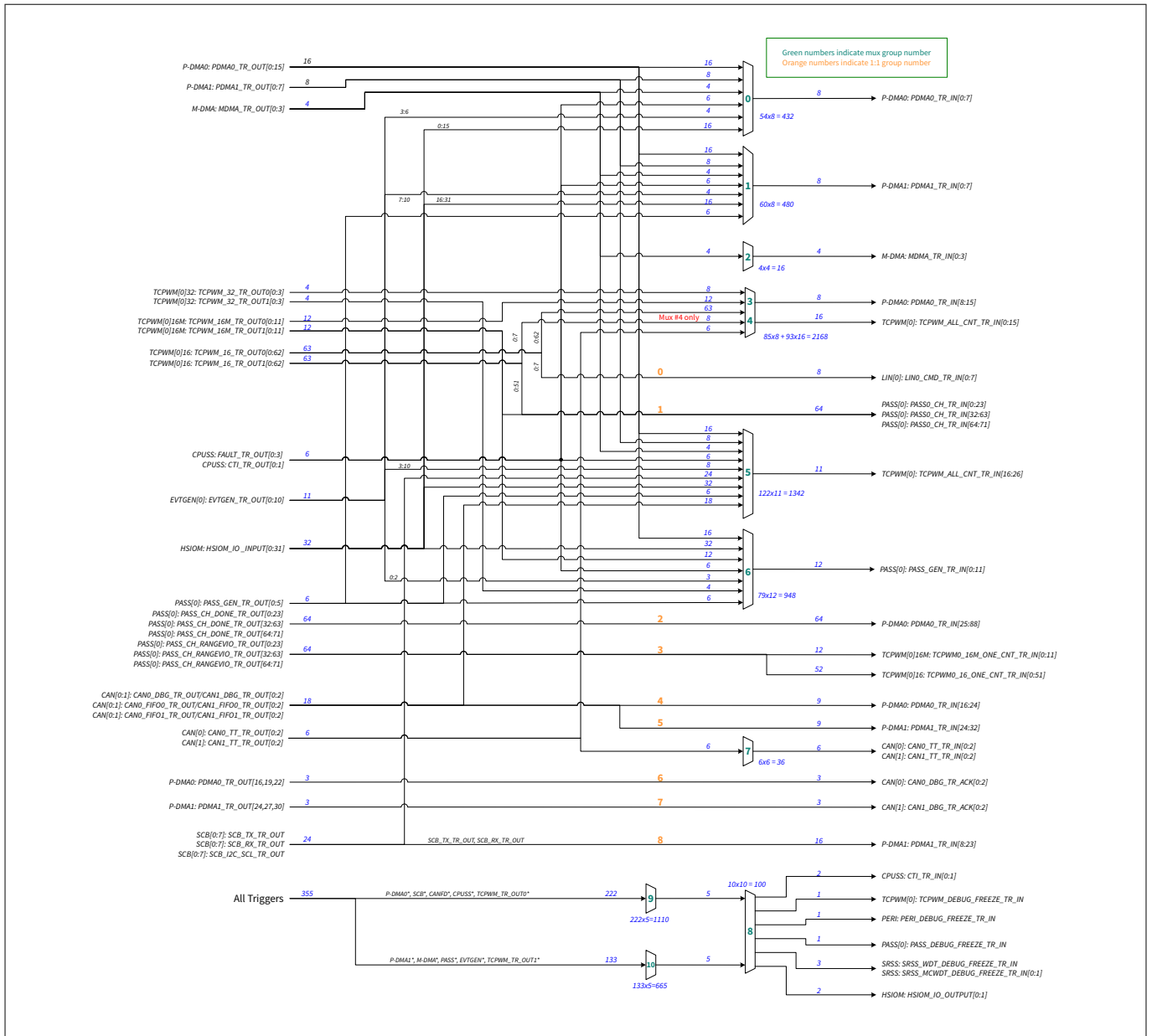
Figure 14 Trigger multiplexer 15)
