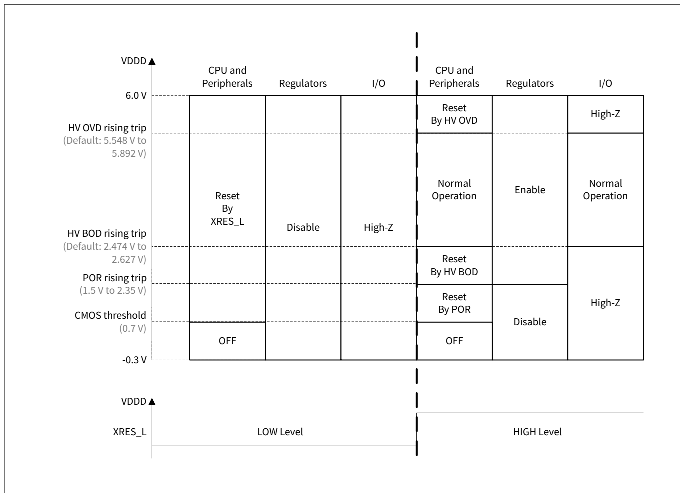
Figure 28 Device operations supply range
