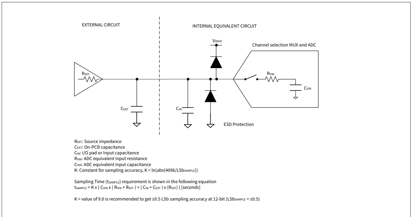
Figure 20 ADC equivalent circuit for analog input
