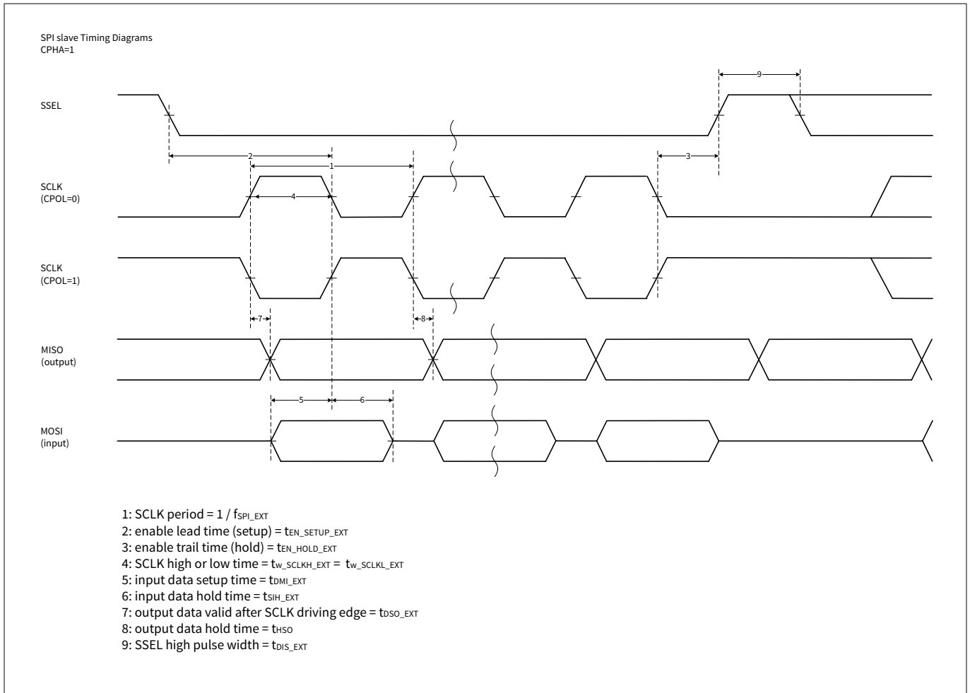
Figure 27 SPI slave timing diagrams with HIGH clock phase
