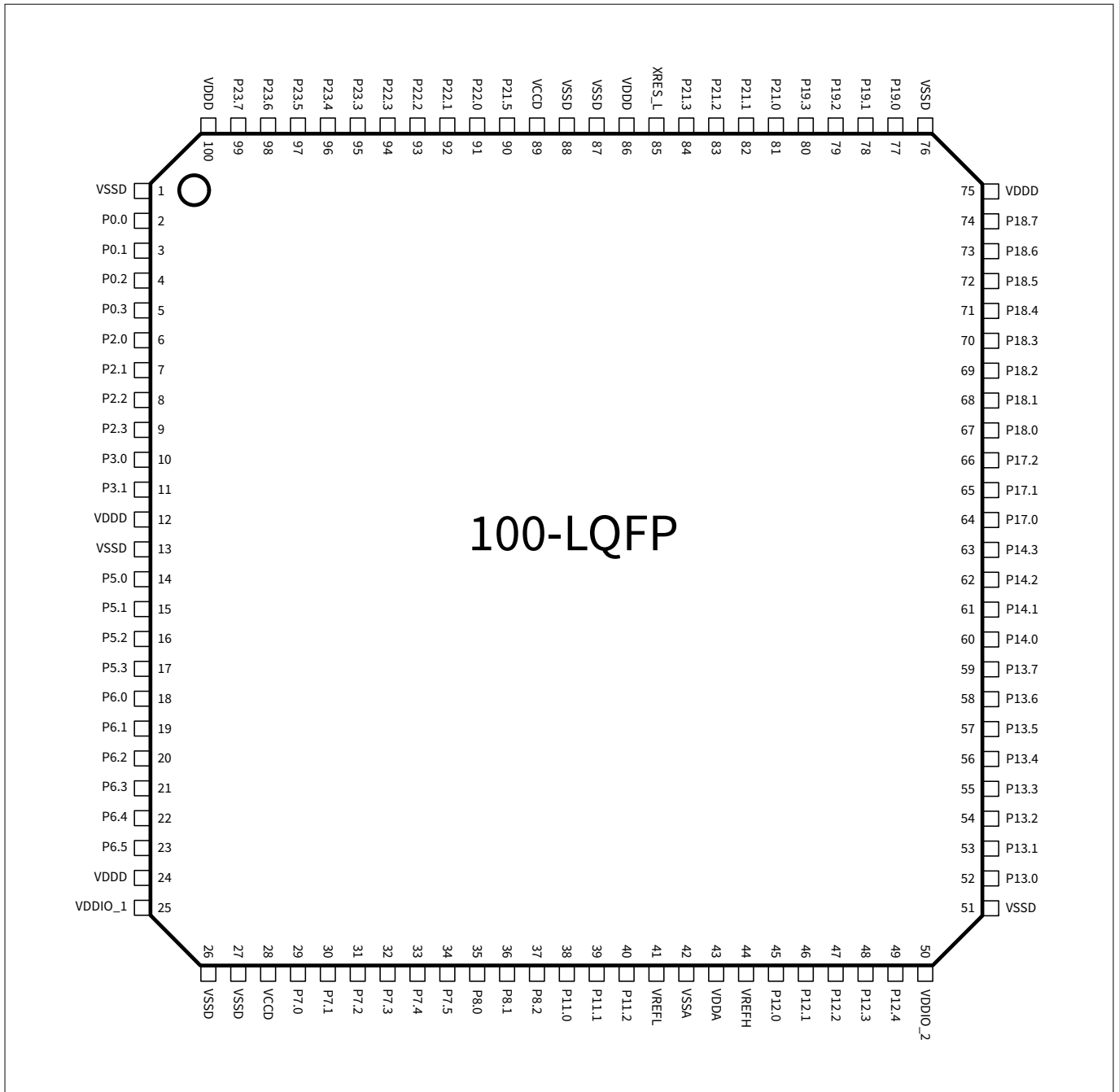
Figure 8 100-LQFP pin assignment
