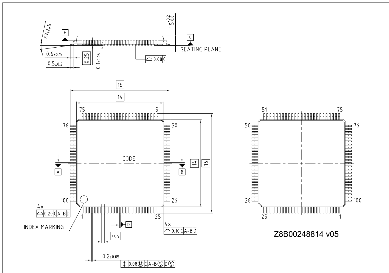
Figure 42 100-LQFP package outline (PG-LQFP-100)
