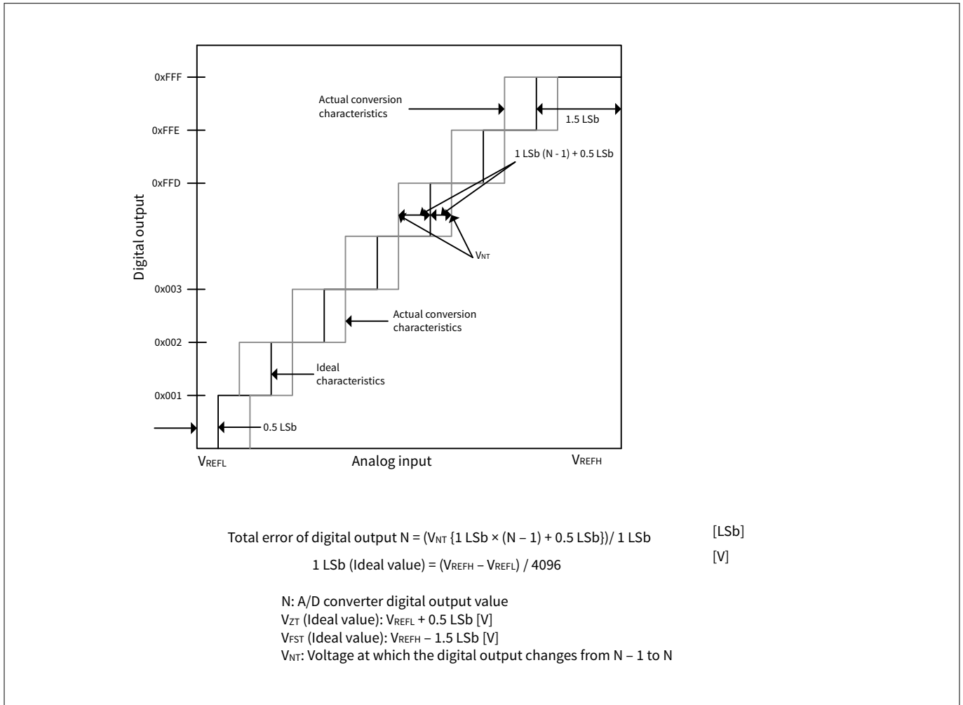
Figure 18 ADC characteristics and error definitions
