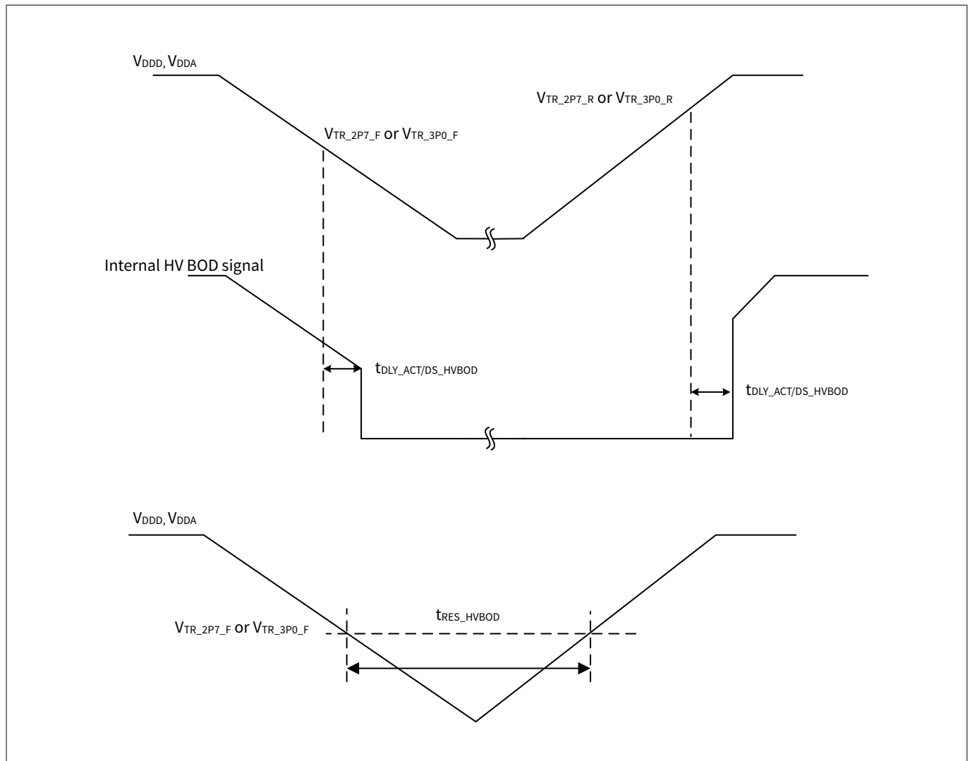
Figure 30 High-voltage BOD specifications
