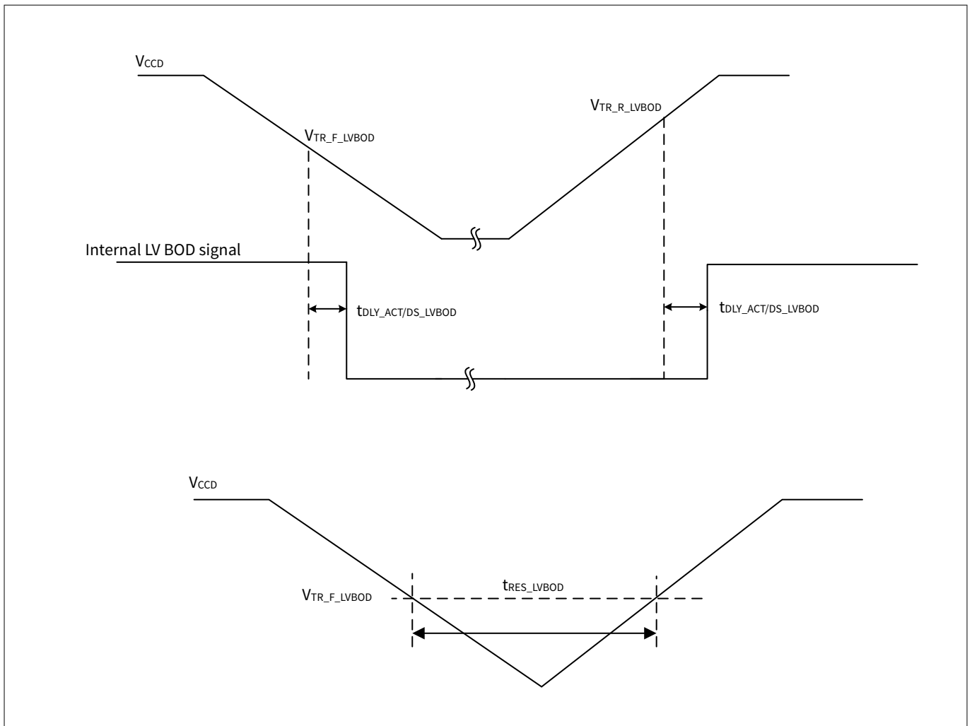
Figure 31 Low-voltage BOD specifications
