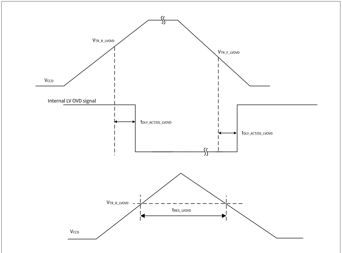
Figure 33 Low-voltage OVD specifications
