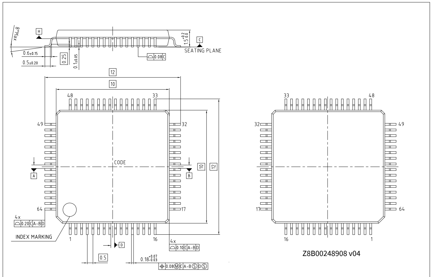
Figure 44 64-LQFP package outline (PG-LQFP-64)
