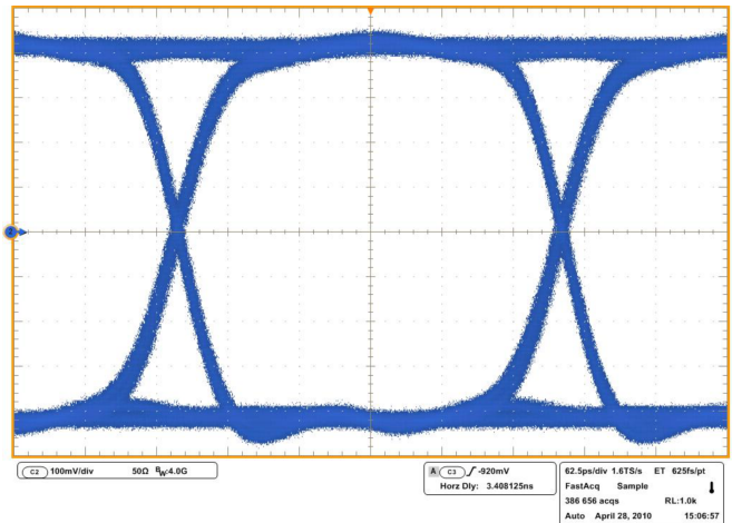
H: 62.5 ps / div, V: 100 mV / div (BNC_IO Output Shown)
