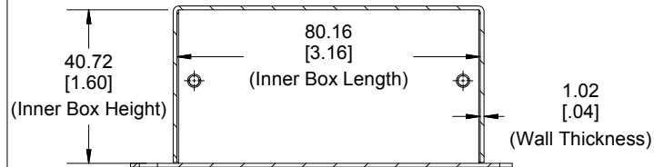
SECTION B-B Side View of Assembly
