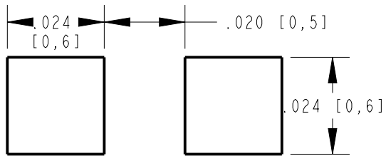
RECOMMENDED SOLDER PAD LAYOUT
