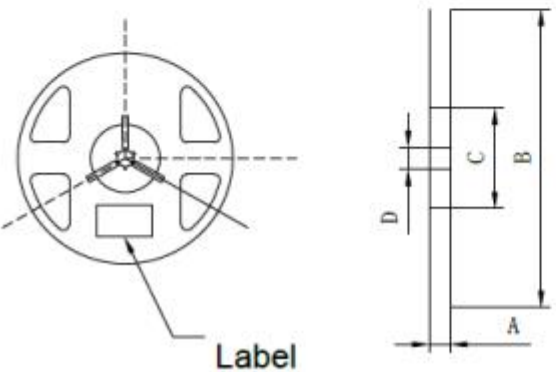
Reel Dimension
