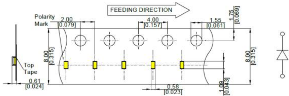
Carrier Tape Dimension
