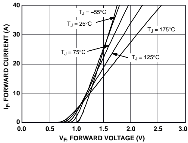
Figure 1. Forward Characteristics
