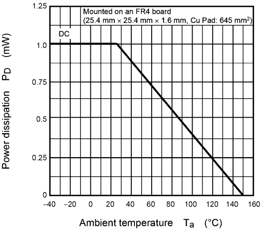
Fig. 8.14 P_D - T_a
