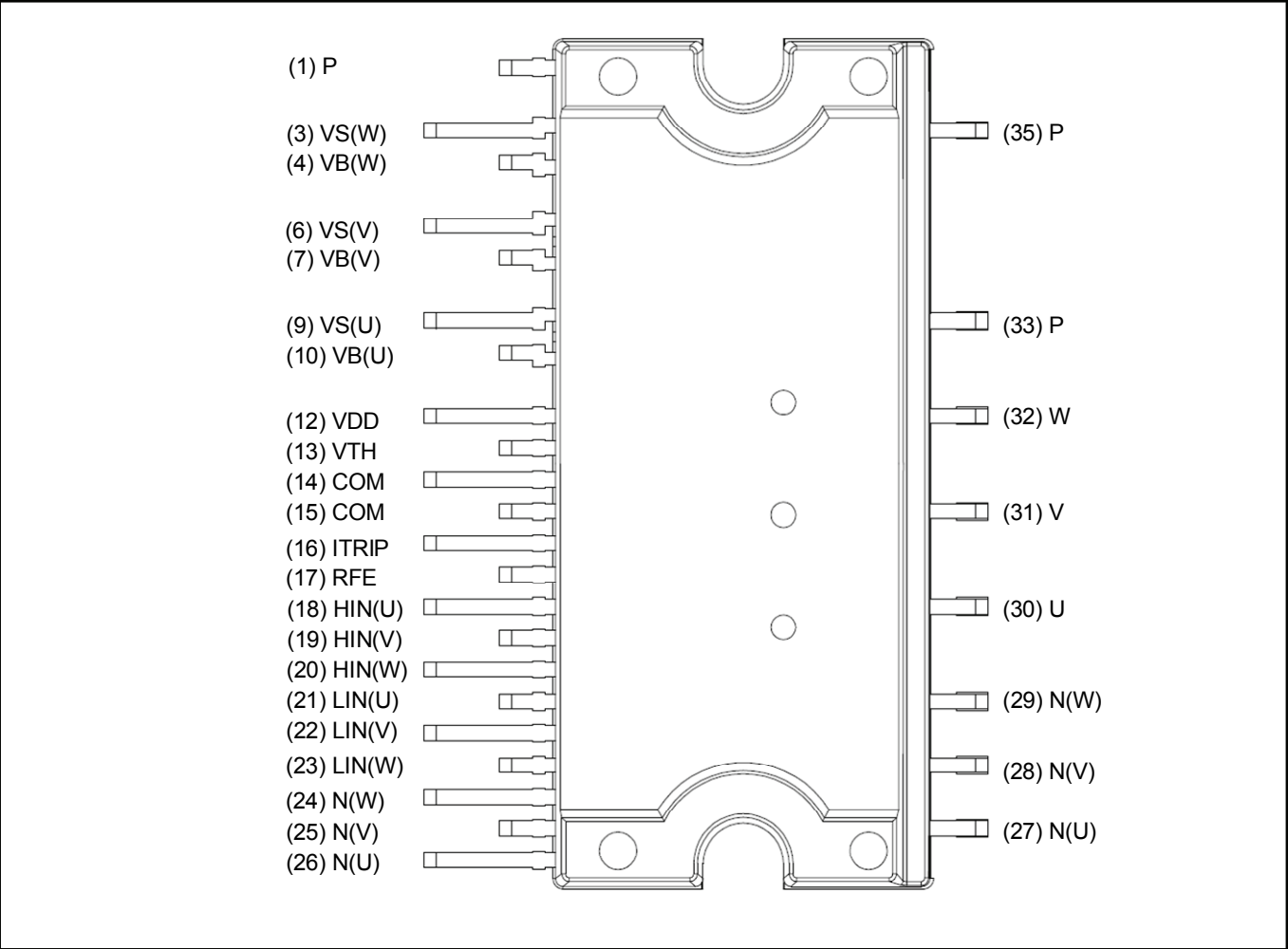
Figure 2 Pin configuration
