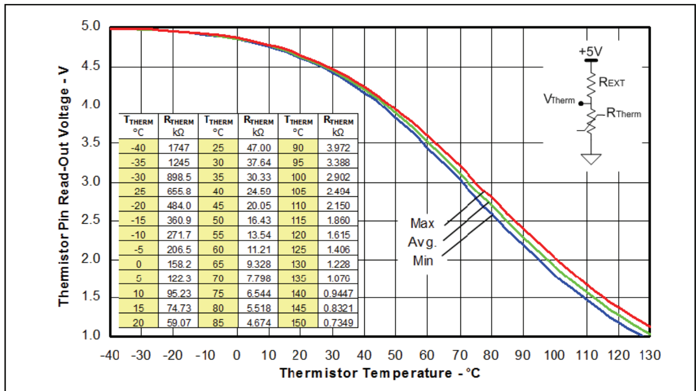
Figure 7 Thermistor readout vs. temperature (with 4.7kohm R_{EXT} pull-down resistor) and typical thermistor resistance values vs. temperature table
