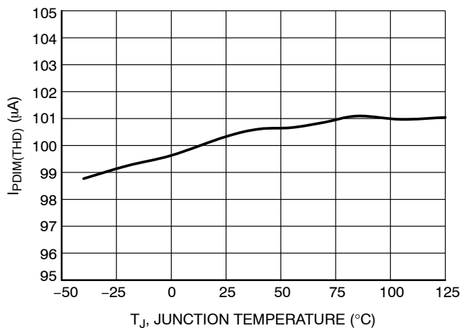
Figure 21. I PDIM(THD) vs. Junction Temperature
