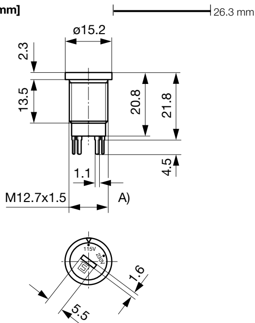
Drilling diagram
