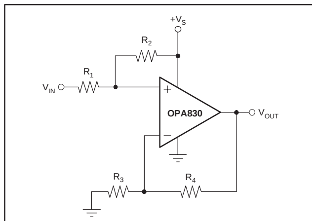
Figure 4. DC Level-Shifting
