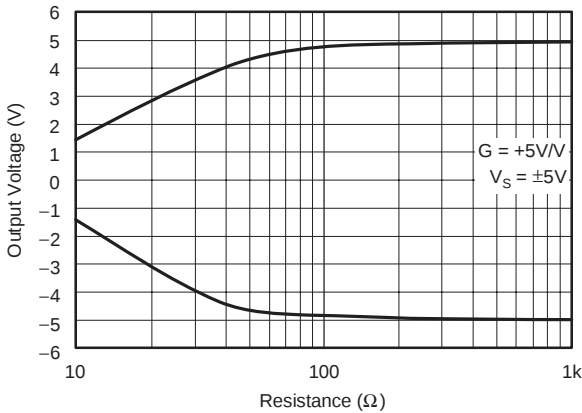
OUTPUT SWING vs LOAD RESISTANCE
