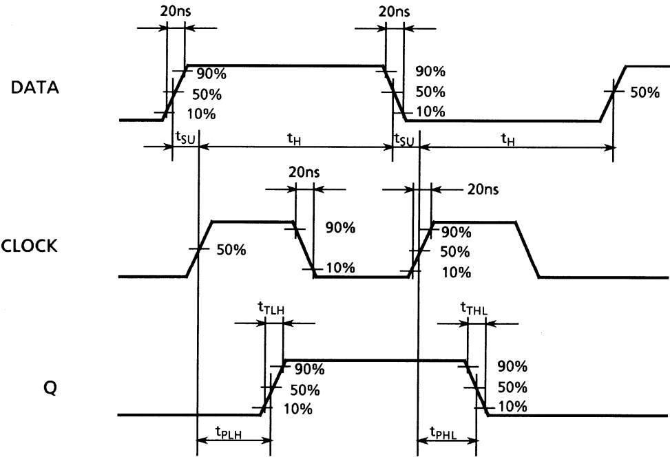
Waveform 1
