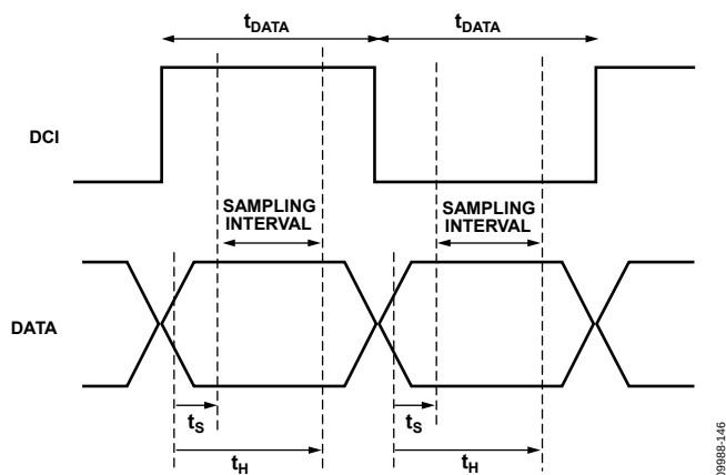
Figure 44. Timing Diagram for Input Data Port
