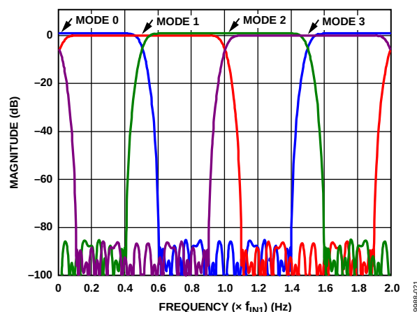
Figure 50. HB1 Filter Modes
