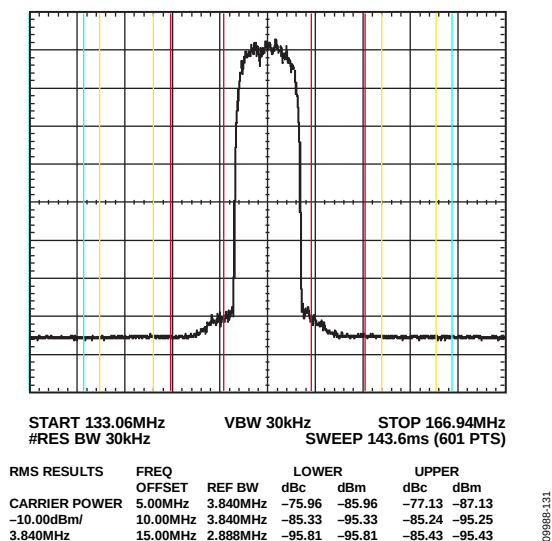
Figure 35. One-Carrier W-CDMA ACLR Performance, IF = ~150 MHz
