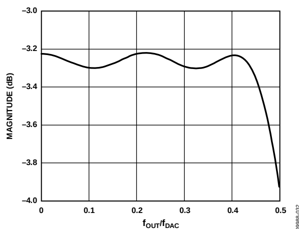
Figure 61. Sample Composite Responses of the \text{Sinc}^{-1} Filter with \sin(x)/x Roll-Off
