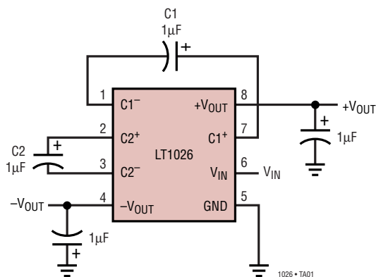
Voltage Doubler and Inverter
