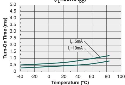
Typical Turn-On Time vs. Temperature ( I_L = 50\text{mA}_{DC} )
