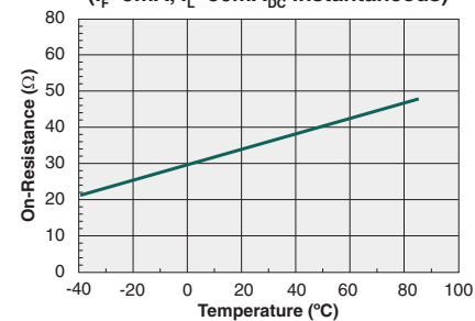
Typical On-Resistance vs. Temperature ( I_F = 5\text{mA} , I_L = 50\text{mA}_{DC} Instantaneous)
