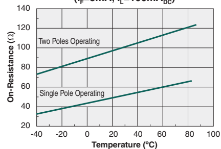
Typical On-Resistance vs. Temperature ( I_F = 5\text{mA} , I_L = 100\text{mA}_{DC} )
