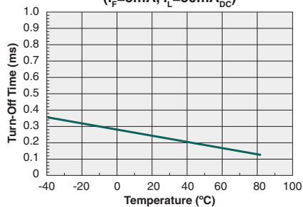
Typical Turn-Off Time vs. Temperature ( I_F = 5\text{mA} , I_L = 50\text{mA}_{DC} )
