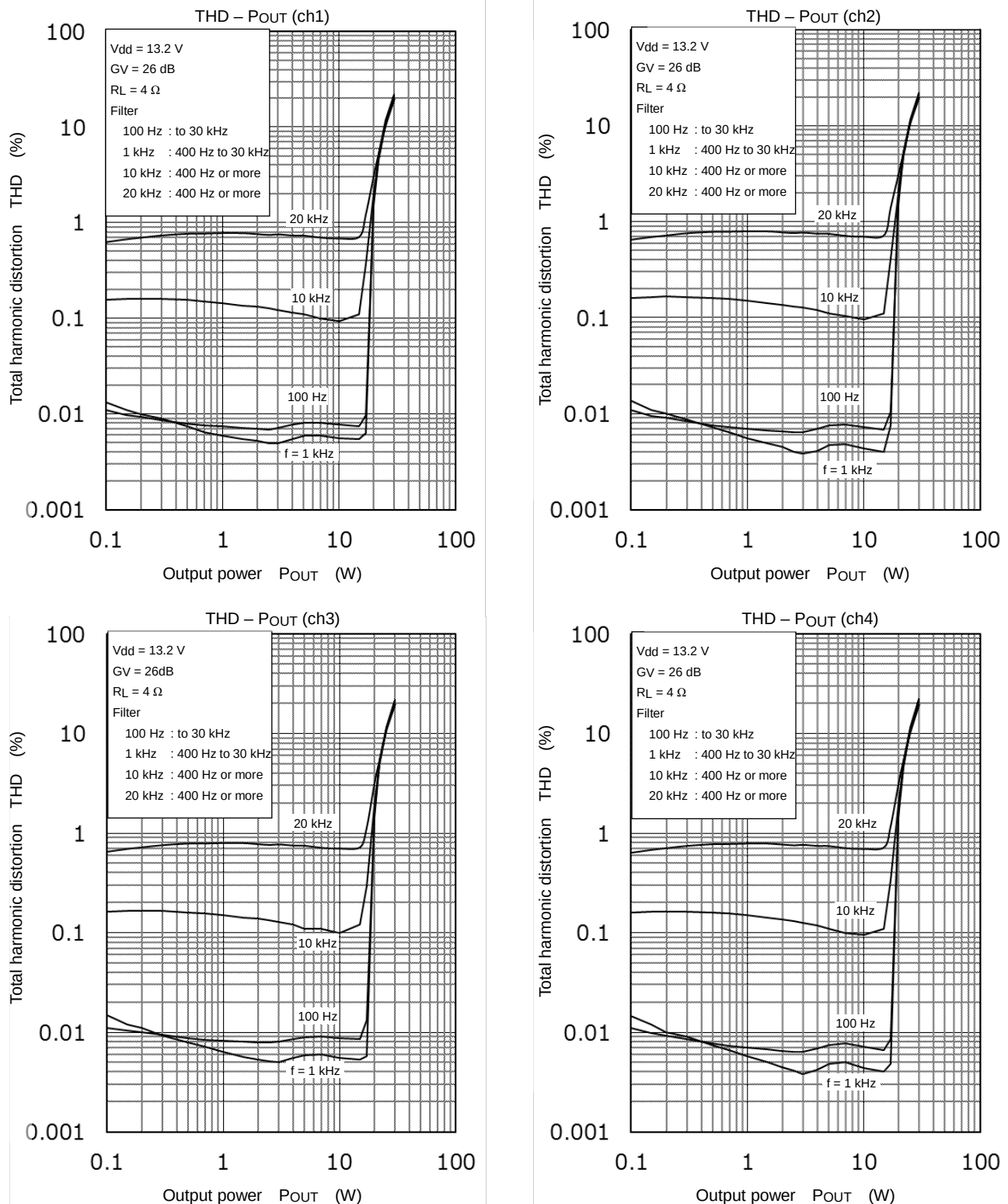
Figure 13-1 Total Harmonic Distortion of Each Frequency (RL = 4 \Omega )
