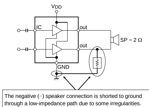
Figure 11 Layer Short
