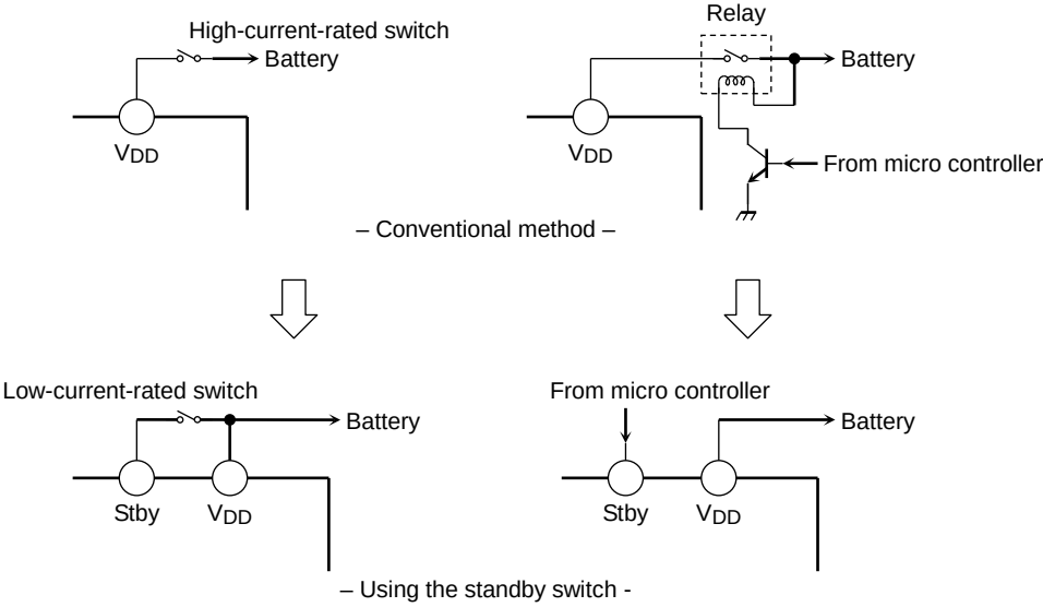
Figure 2 Standby switch
