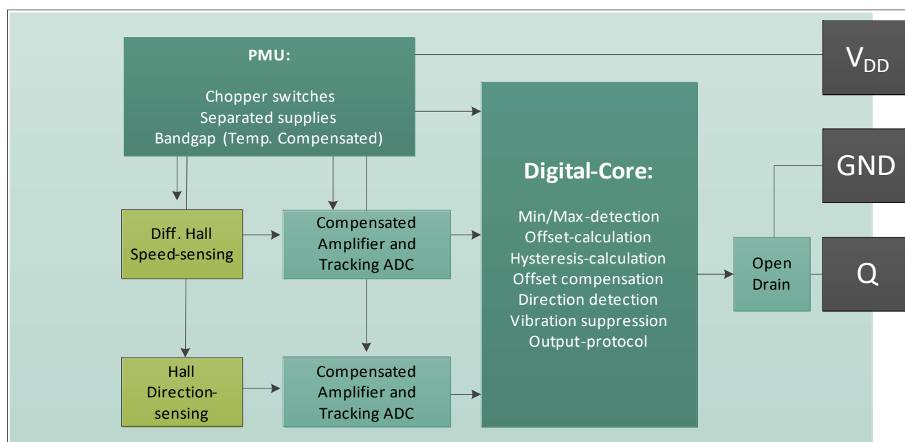
Figure 3 Block Diagram
