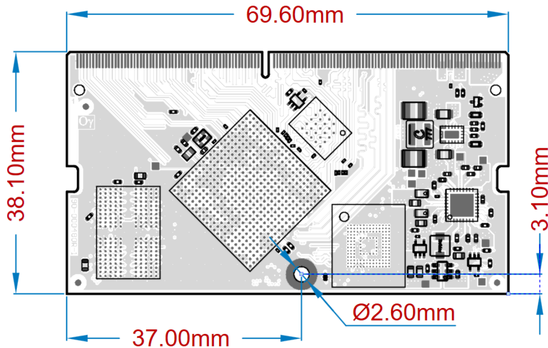
Figure 3 MitySOM-AM62A Mechanical Outline (View From Top)
