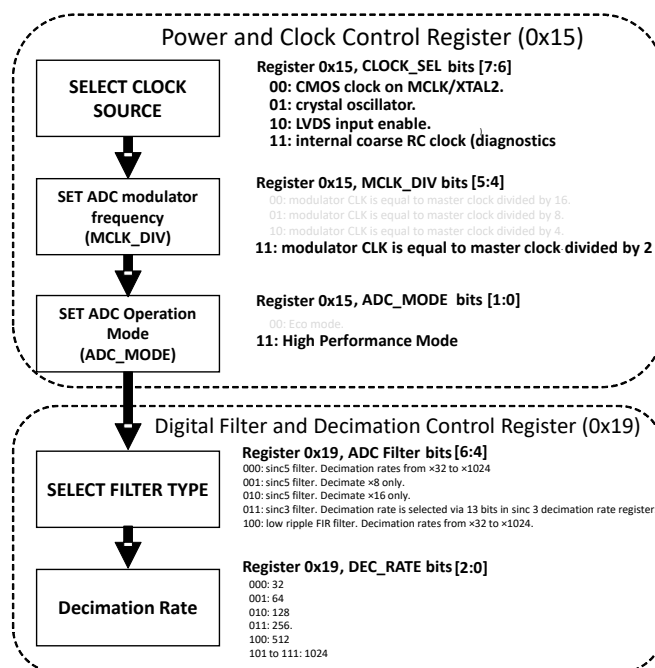
Figure 12. Basic Register Setup for ADAQ7768-1
