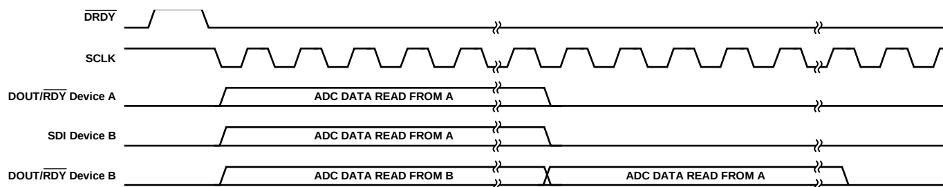
Figure 94. Data Output Format When Devices Daisy-Chained ( \overline{\text{PIN}} Control Mode Only)
