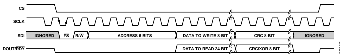
Figure 101. Data Output Format When Using CRC
