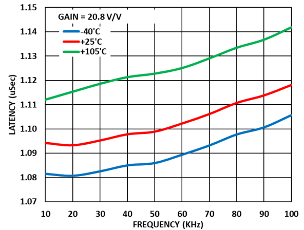
Figure 47. Analog Front End (AFE) Latency vs Frequency across Temperature, Gain = 20.8 V/V
