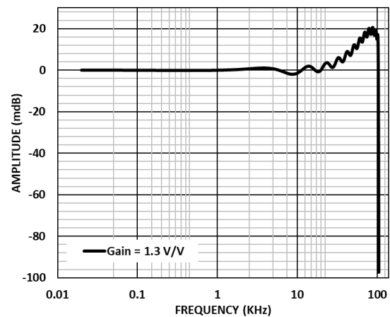
Figure 85. ADAQ7768-1 Wideband Low Ripple FIR Filter Magnitude Flatness, Gain = 1.3 V/V Normalized. 256 kSPS ODR
