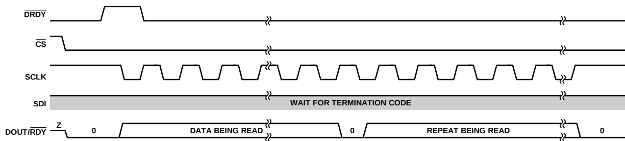
Figure 103. Continuous ADC Read Data Format with \overline{\text{RDY}} Function Disabled
