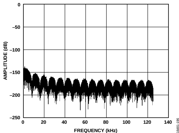
Figure 110. Example Filter Profile Upload
