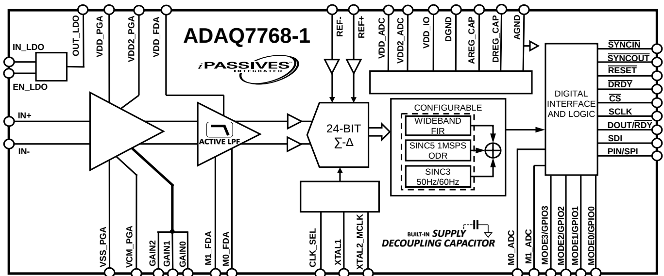
Figure 1. Block Diagram
