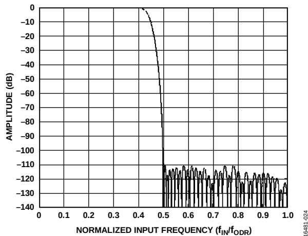
Figure 82. Low Ripple FIR Filter Frequency Response
