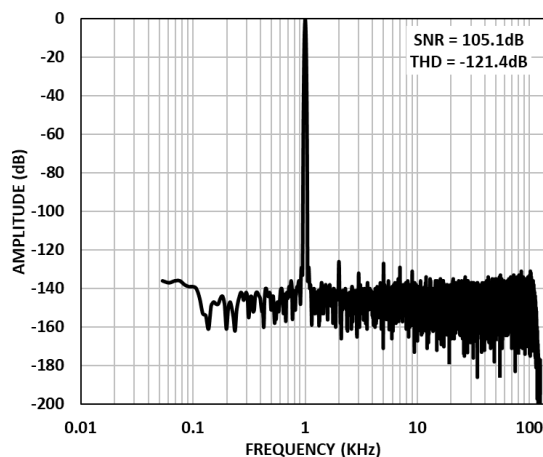
Figure 15. FFT Wideband Low Ripple FIR Filter, Differential Input, -0.5dBFS, Gain = 0.65 V/V, FDA = Full Power.
