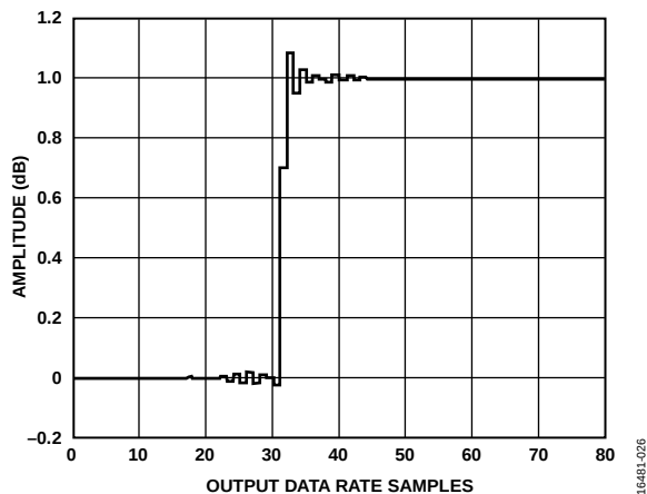
Figure 84. Wideband Low Ripple FIR Filter Step Response
