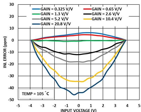
Figure 29. INL Error vs. Input Voltage for Various Gain, Differential Input at 105 °C
