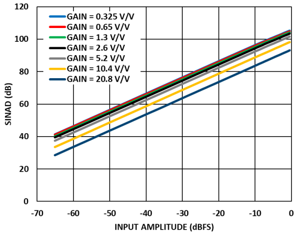
Figure 34. SINAD across Input Amplitude at Various Gain, 1KHz, FDA = Full Power.
