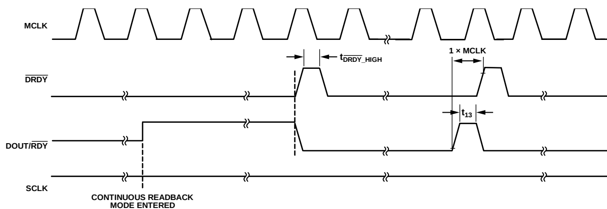
Figure 6. DOUT/ \overline{RDY} Behavior Without SCLK Applied
