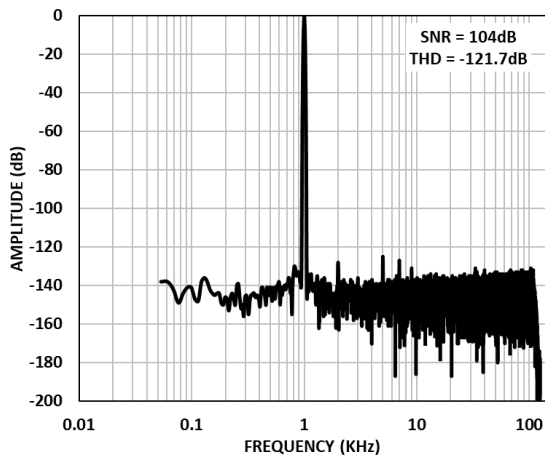
Figure 20. FFT Wideband Low Ripple FIR Filter, Bipolar Single Ended Input, -0.5dBFS, Gain = 1.3 V/V, FDA = Full Power.
