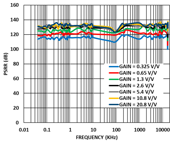
Figure 51. LDO AC PSRR across All Gains, connected to VDD2_PGA, VDD_FDA, VDD_ADG, VDD2_ADC with Internal Supply Decoupling Capacitor
