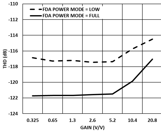
Figure 33. THD vs. Gain over FDA Power Mode, -0.5dBFS, 1kHz.
