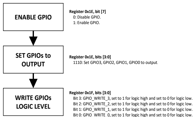
Figure 11. GPIO Gain Control Flow Chart
