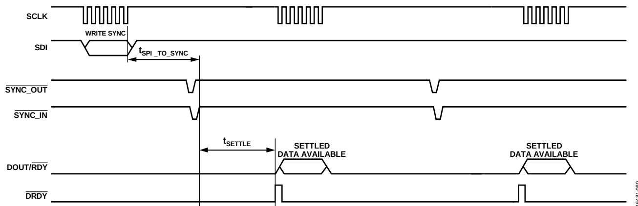
Figure 106. One Shot Conversion Mode, SYNC_IN Pulse Initiated by a Register Write
