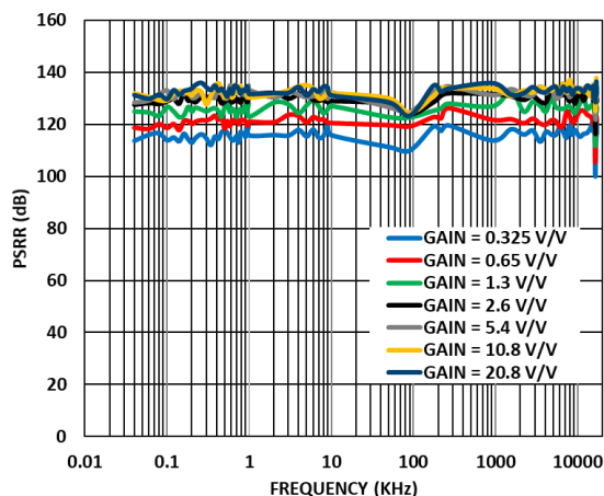
Figure 78. LDO AC PSRR, using internal decoupling capacitor of VDD2_PGA, VDD_FDA, VDD_ADC, VDD2_ADC
