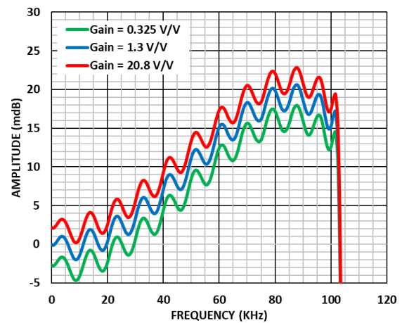
Figure 49. ADAQ7768-1 Wideband Low Ripple FIR Filter Pass-Band Ripple, ODR = 256 kSPS, Normalized to Gain = 1.3 V/V
