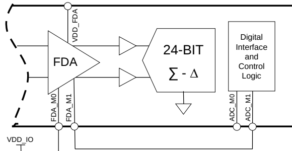
Figure 72. FDA Full Power Mode Connection
