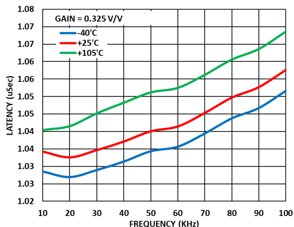
Figure 41. Analog Front End (AFE) Latency vs Frequency across Temperature, Gain = 0.325 V/V
