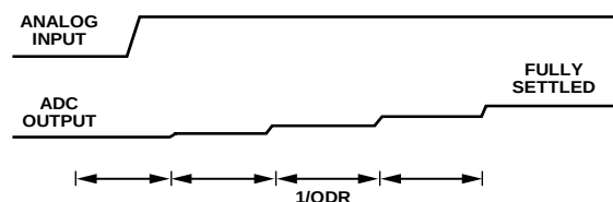
Figure 88. Sinc5 Filter Step Response
