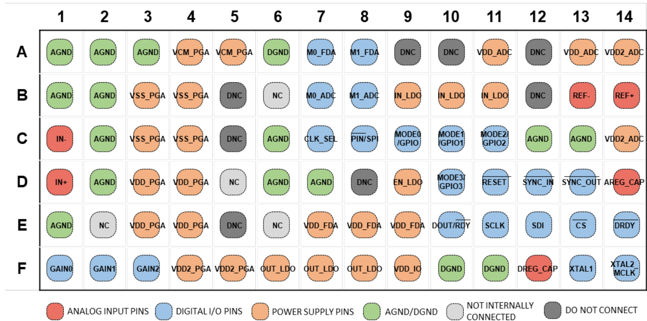
Figure 13. Pin Configuration
