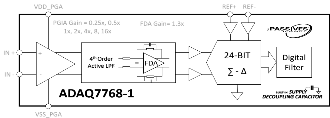
Figure 65. ADAQ7768-1 Top Level Core Signal Chain
