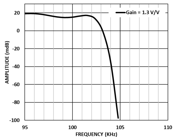
Figure 86. ADAQ7768-1 Wideband Low Ripple FIR Filter, -0.1dB Pass Band
