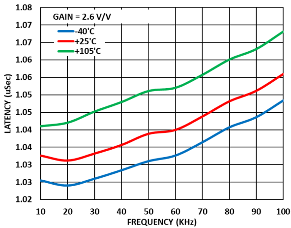
Figure 44. Analog Front End (AFE) Latency vs Frequency across Temperature, Gain = 2.6 V/V
