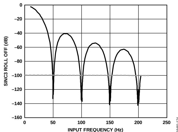
Figure 90. Sinc3 Filter Frequency Response Showing 50 Hz Rejection, 50 Hz ODR, \times 163,840 Decimation
