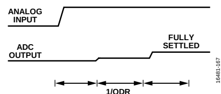
Figure 89. Sinc3 Filter Step Response
