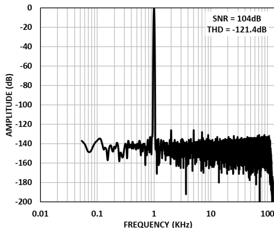
Figure 16. FFT Wideband Low Ripple FIR Filter, Differential Input, -0.5dBFS, Gain = 1.3 V/V, FDA = Full Power.
