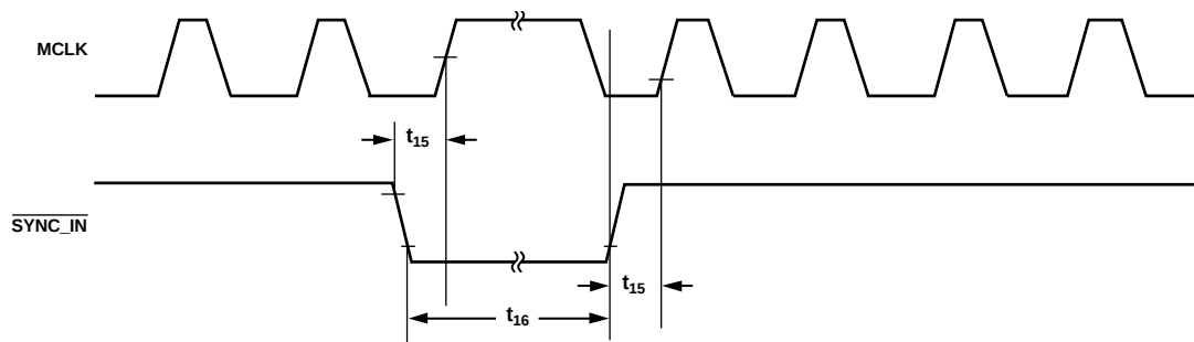
Figure 7. Synchronous \overline{SYNC\_IN} Pulse
