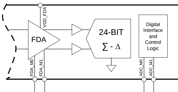
Figure 71. FDA Eco Power Mode Connection
