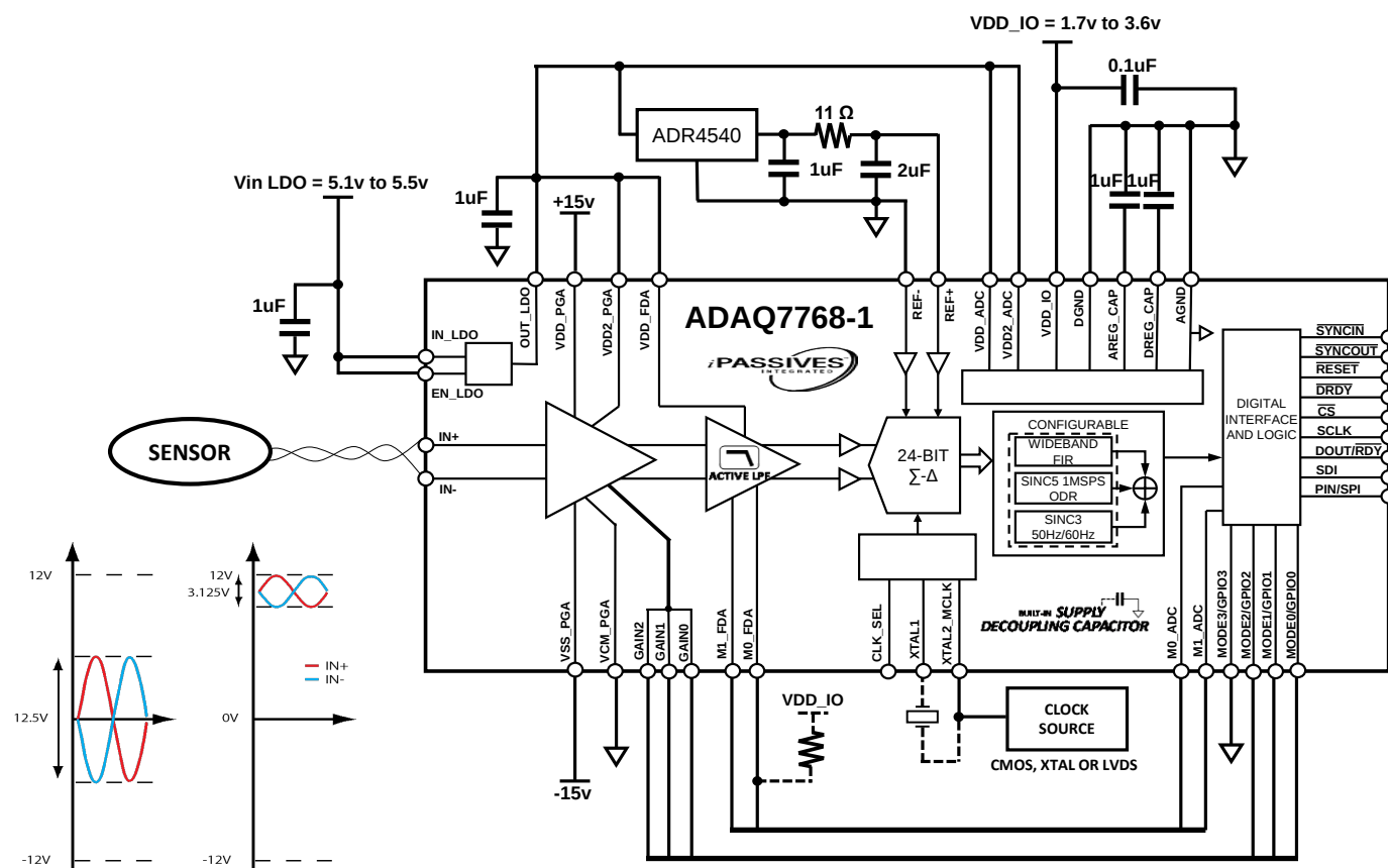
Figure 9. Typical Connection Diagram
