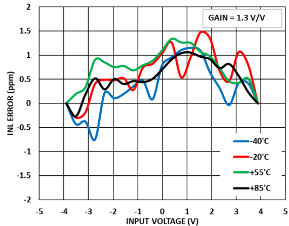
Figure 24. INL Error vs. Input Voltage over Temperature, Differential Input, Gain = 1.3 V/V.
