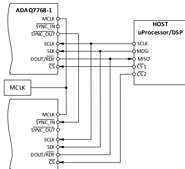
Figure 95. Basic SPI Synchronization Diagram
