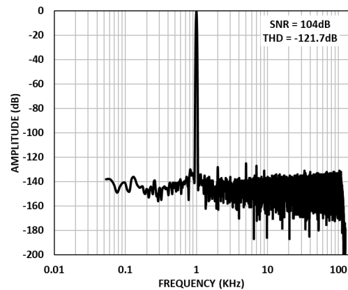
Figure 59. Bipolar Single-ended input, IN+ = -0.5dBFS 1kHz Bipolar Sine, IN- = 0V, 32k Point FFT, ODR= 256 kSPS, VREF=4.096V, Gain = 0.325V/V.
