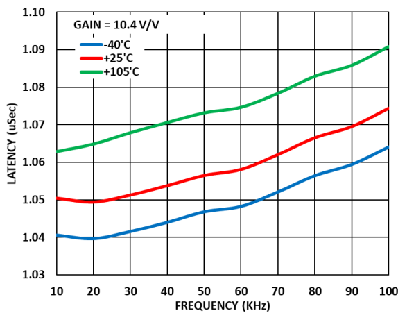
Figure 46. Analog Front End (AFE) Latency vs Frequency across Temperature, Gain = 10.4 V/V
