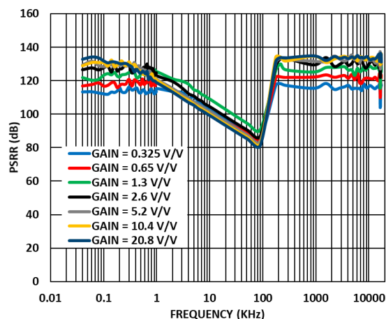
Figure 79. VDD_PGA AC PSRR vs all gains, using the internal 0.1uF supply decoupling capacitor
