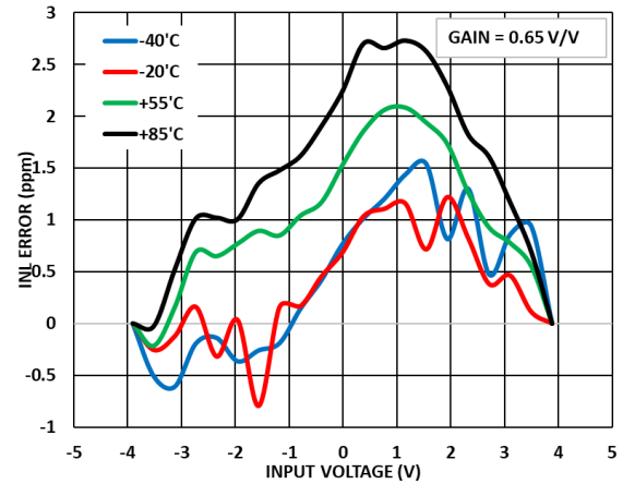
Figure 23. INL Error vs. Input Voltage over Temperature, Differential Input, Gain = 0.65 V/V.
