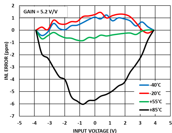
Figure 26. INL Error vs. Input Voltage over Temperature, Differential Input, Gain = 5.2 V/V
