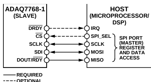
Figure 96. Basic Serial Port Connection Diagram
