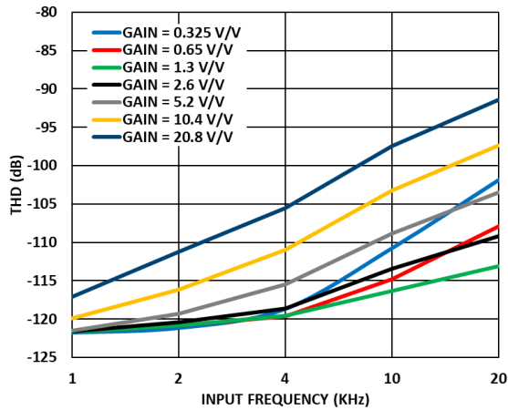
Figure 32. THD vs. Input Frequency for Various Gain, -0.5dBFS, FDA = Full Power.
