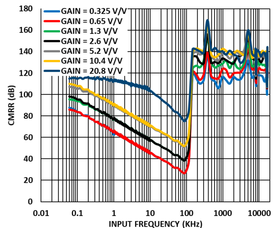
Figure 55. ADAQ7768-1 AC CMRR across all gains
