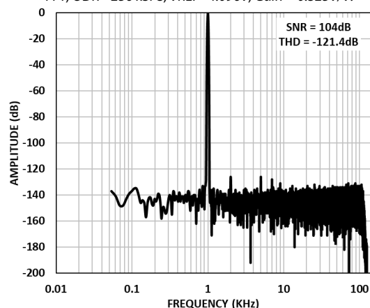
Figure 62. Fully differential input, -0.5dBFS 1kHz Sine, VCM=0V, 32k Point FFT, ODR= 256 kSPS, VREF=4.096V, Gain = 1.3V/V.
