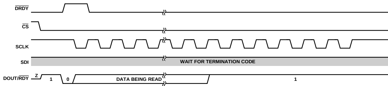
Figure 104. Continuous ADC Read Data Format with \overline{\text{RDY}} Function Enabled on the DOUT/ \overline{\text{RDY}} Pin
