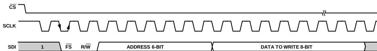
Figure 99. 3-Wire SPI Write Frame ( \overline{\text{CS}} = 0 )
