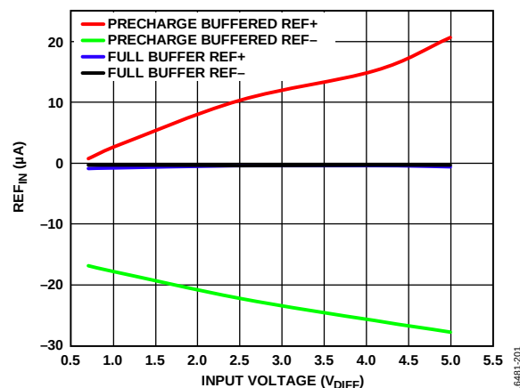
Figure 74. Reference Input Current ( \text{REF}_{\text{IN}} ) vs. Input Voltage, Precharge Buffered REF+ and REF- and Full Buffer REF+ and REF-
