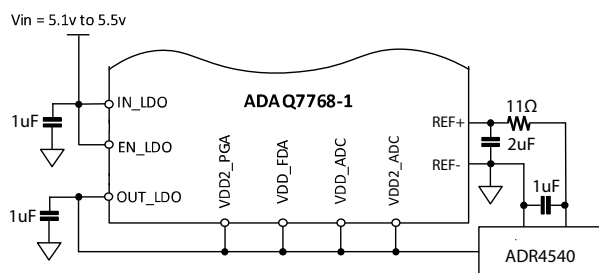
Figure 76. ADAQ7768-1 power supply connection using internal LDO
