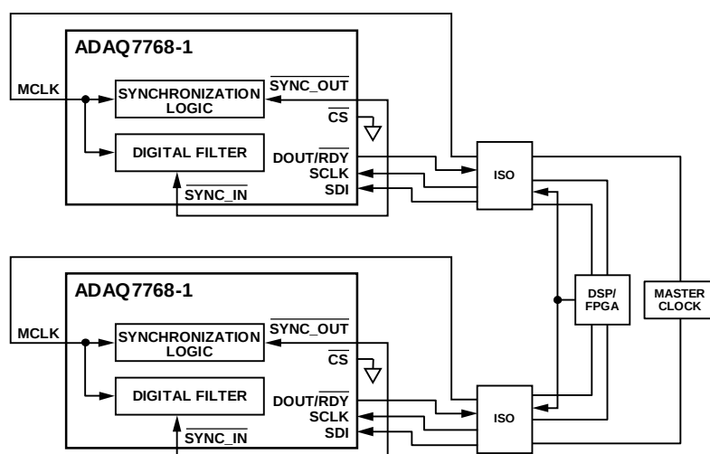
Figure 107. Synchronization in Channel to Channel Isolated Systems
