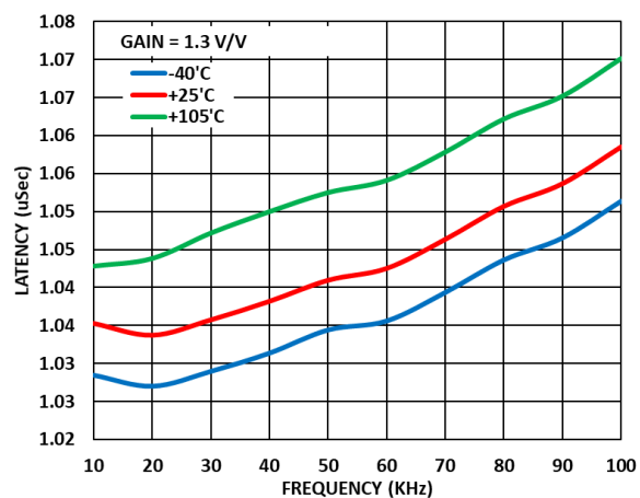
Figure 43. Analog Front End (AFE) Latency vs Frequency across Temperature, Gain = 1.3 V/V
