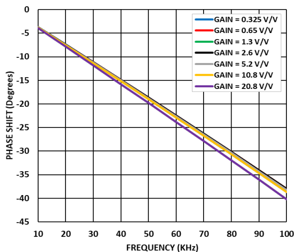
Figure 40. Analog Front End (AFE) Phase Response
