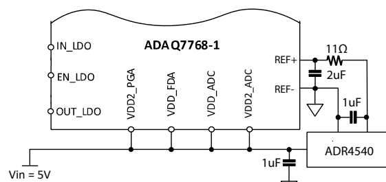
Figure 77. Float IN_LDO and OUT_LDO pins when not used
