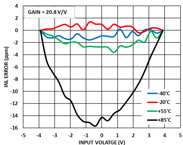
Figure 28. INL Error vs. Input Voltage over Temperature, Differential Input, Gain = 20.8 V/V
