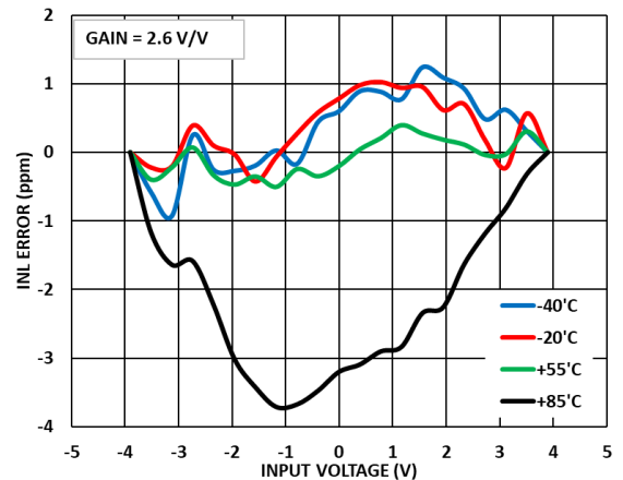
Figure 25. INL Error vs. Input Voltage over Temperature, Differential Input, Gain = 2.6 V/V.
