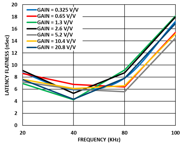
Figure 48. Analog Front End (AFE) Latency Flatness vs Frequency across Gain, Normalized to Latency at 10kHz
