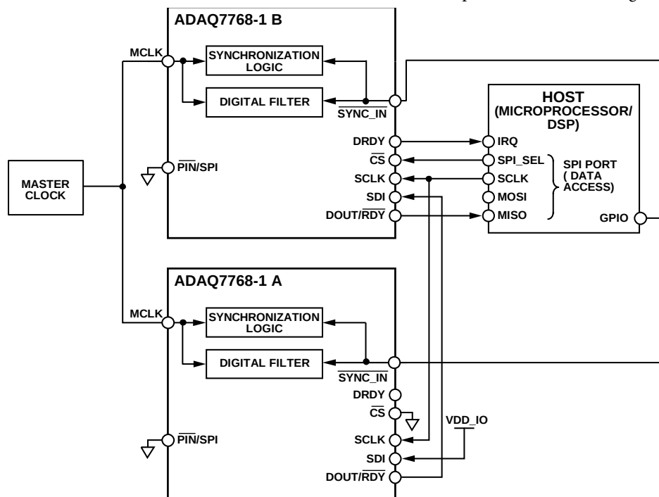
Figure 93. Daisy-Chaining Multiple ADAQ7768-1 Devices
