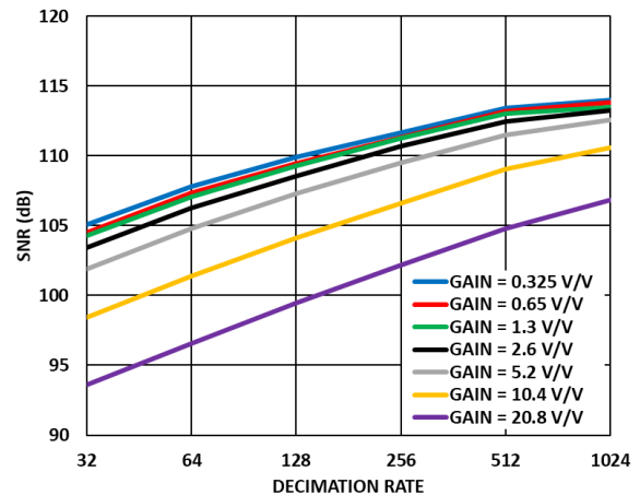
Figure 37. SNR vs Decimation Rate at Various Gain, Wideband Low Ripple FIR Filter, 0.5dBFS, 1KHz.
