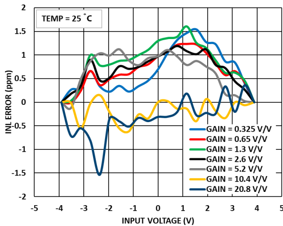
Figure 21. INL Error vs. Input Voltage for Various Gain, Differential Input at 25°C.
