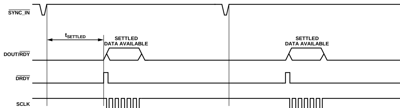
Figure 105. One Shot Conversion Mode, \overline{\text{SYNC\_IN}} Pin Driven with an External Source
