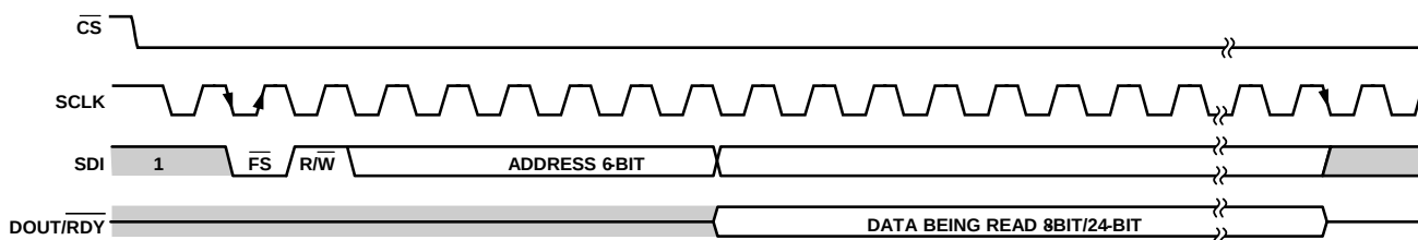
Figure 100. 3-Wire SPI Read Frame ( \overline{\text{CS}} = 0 )
