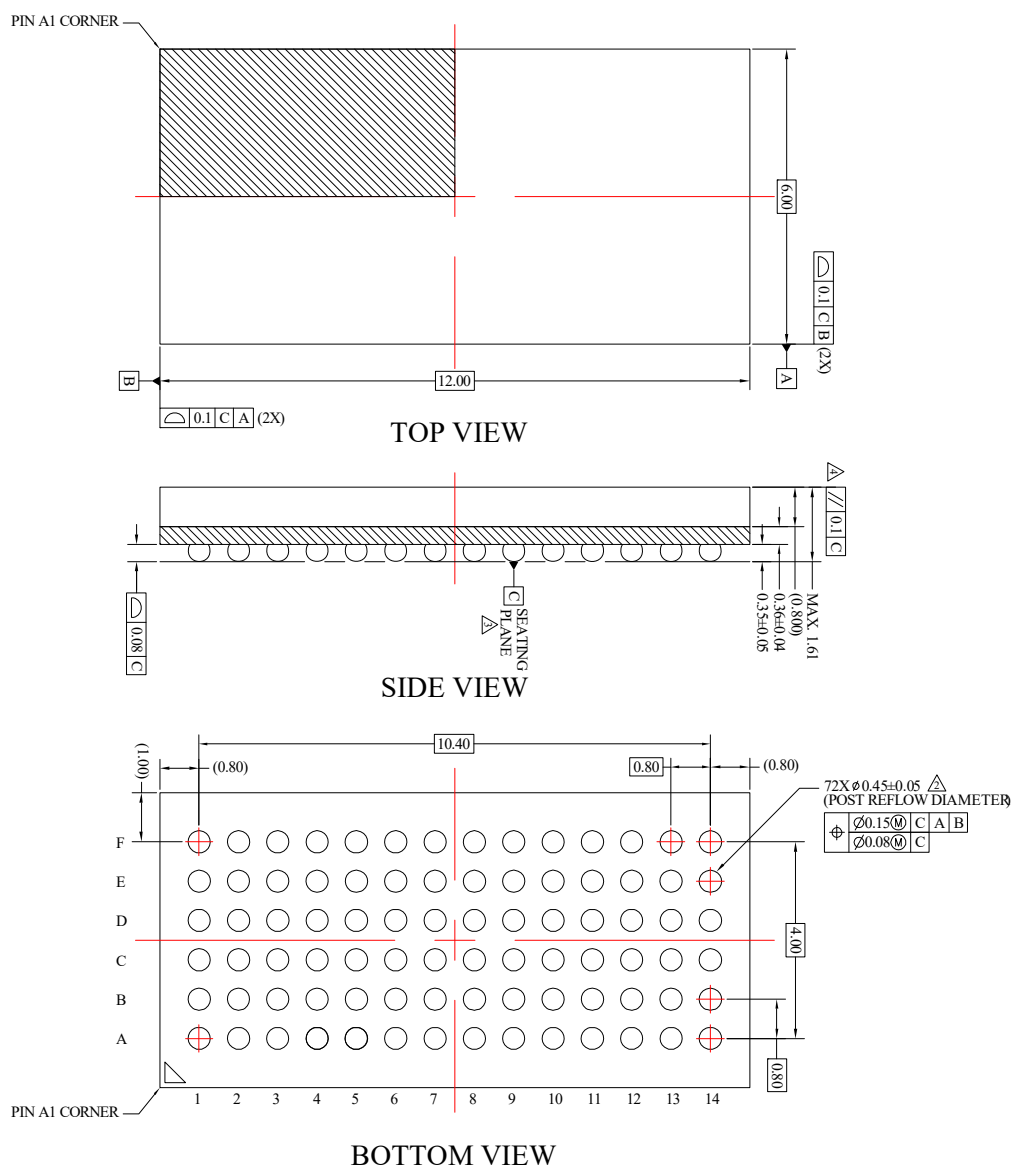
Figure 111. Package Drawings
