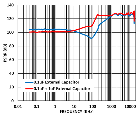
Figure 81. VDD_IO AC PSRR using 0.1uF and additional 1uF supply decoupling capacitor
