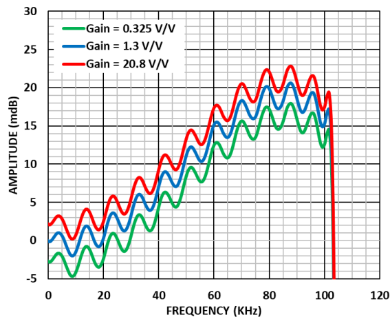
Figure 83. ADAQ7768-1 Wideband Low Ripple FIR Filter Pass-Band Ripple, Normalized to Gain = 1.3 V/V
