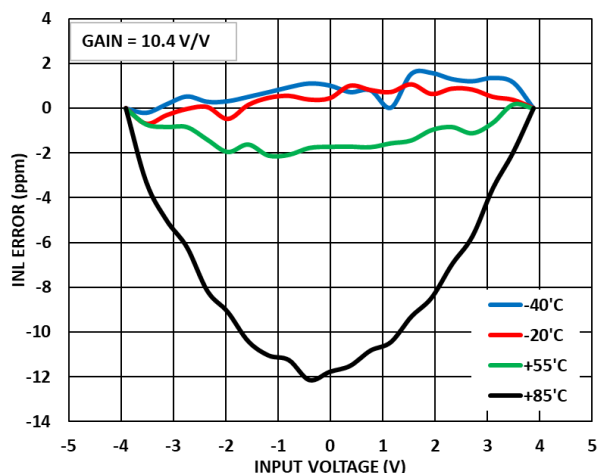
Figure 27. INL Error vs. Input Voltage over Temperature, Differential Input, Gain = 10.4 V/V
