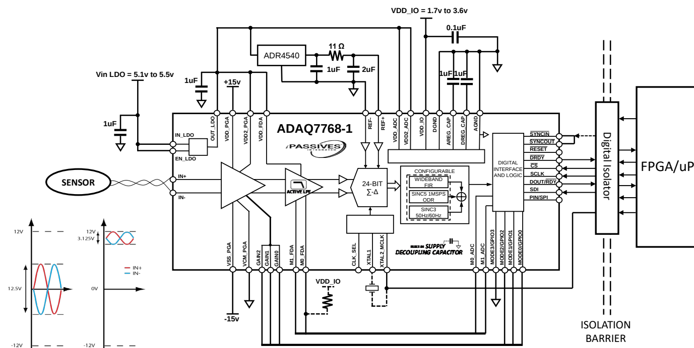
Figure 108. Typical applications diagram of a per channel isolated DAQ system
