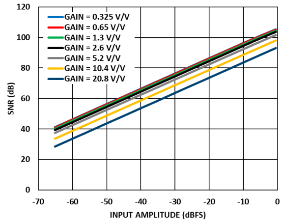
Figure 35. SNR across Input Amplitude at Various Gain, 1KHz.
