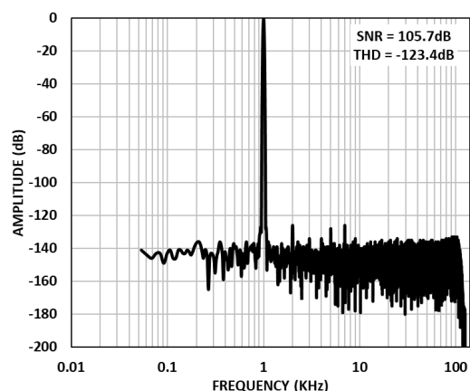
Figure 61. Fully differential input, -0.5dBFS 1kHz Sine, VCM=0V, 32k Point FFT, ODR= 256 kSPS, VREF=4.096V, Gain = 0.325V/V.
