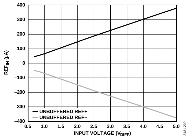
Figure 73. Reference Input Current ( \text{REF}_{\text{IN}} ) vs. Input Voltage, Unbuffered REF+ and REF-
