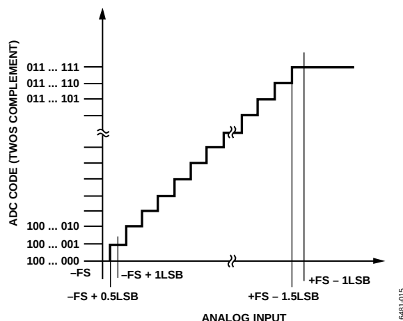
Figure 75. ADC Ideal Transfer Functions (FS is Full-Scale)
