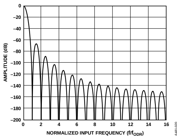
Figure 87. Sinc Filter Frequency Response
