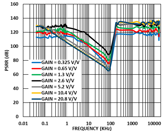
Figure 53. VSS_PGA AC PSRR across All Gains, using the Internal Supply Decoupling Capacitor
