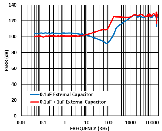
Figure 54. VDD_IO using External Supply Decoupling Capacitor
