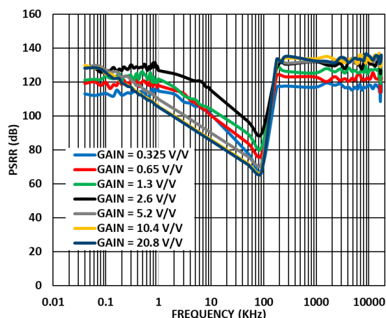
Figure 80. VSS_PGA AC PSRR vs all gains, using the internal 0.1uF supply decoupling capacitor
