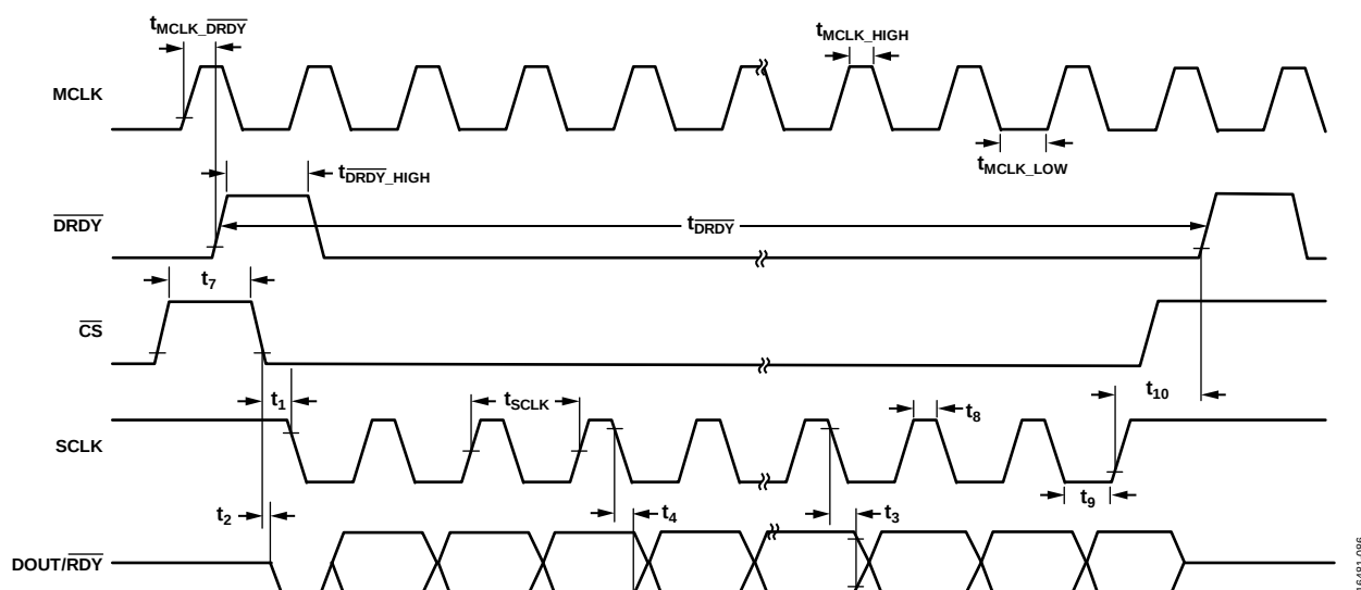
Figure 102. Serial Interface Timing Diagram, Example Reflects Reading an ADC Conversion in Continuous Read Mode
