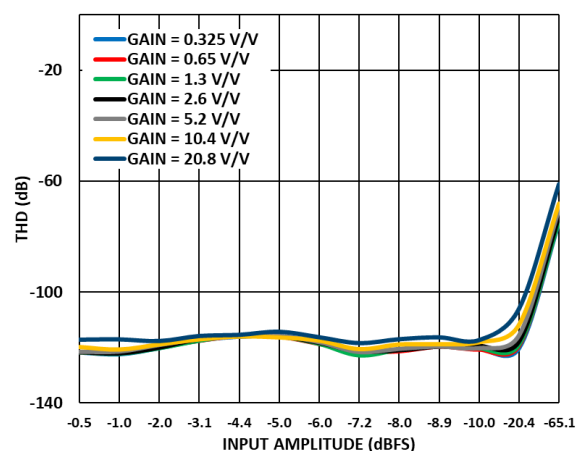
Figure 31. THD across Input Amplitude at Various Gain, 1KHz, FDA = Full Power.
