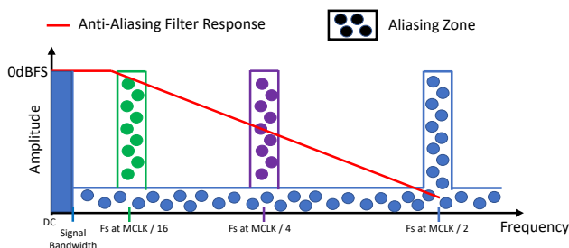
Figure 91. Anti-Alias Filter Response versus MCLK Divider
