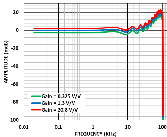
Figure 50. ADAQ7768-1 Magnitude Flatness Response, Wideband Low Ripple FIR Filter, ODR = 256 kSPS, Normalized to Gain = 1.3 V/V
