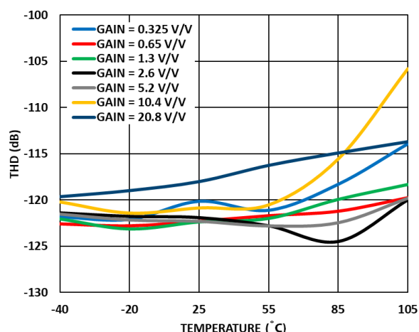
Figure 30. THD across Temperature at Various Gain, -0.5dBFS, 1KHz, FDA = Full Power
