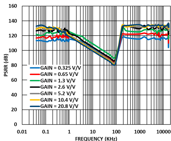
Figure 52. VDD_PGA AC PSRR across All Gains, using the Internal Supply Decoupling Capacitor
