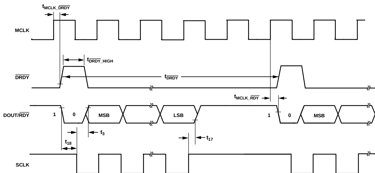
Figure 5. Reading Conversion Result in Continuous Conversion Mode, Continuous Read Mode with \overline{RDY} Enabled ( \overline{CS} Held Low)
