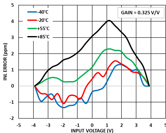
Figure 22. INL Error vs. Input Voltage over Temperature, Differential Input, Gain = 0.325 V/V.
