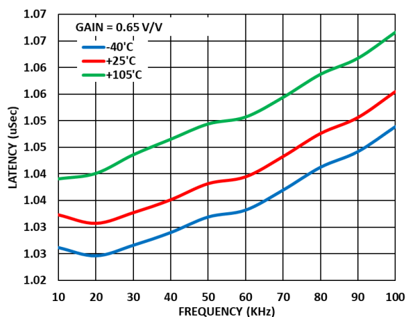
Figure 42. Analog Front End (AFE) Latency vs Frequency across Temperature, Gain = 0.65 V/V
