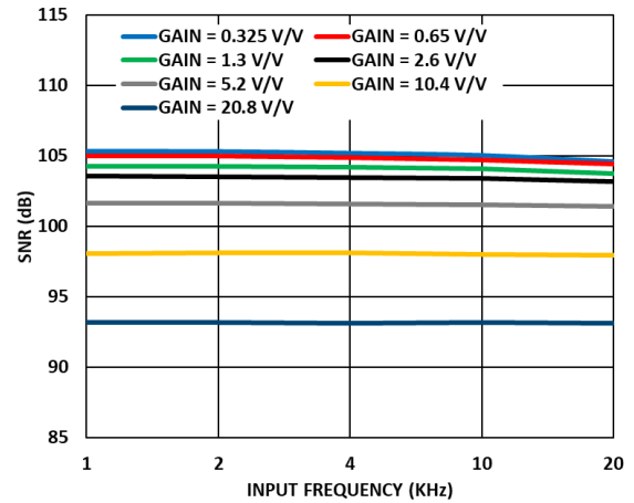
Figure 36. SNR vs. Input Frequency for Various Gain, -0.5dBFS
