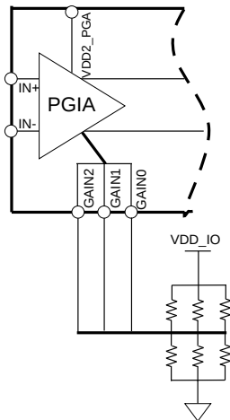
Figure 10. PGIA Gain Control using External Resistors
