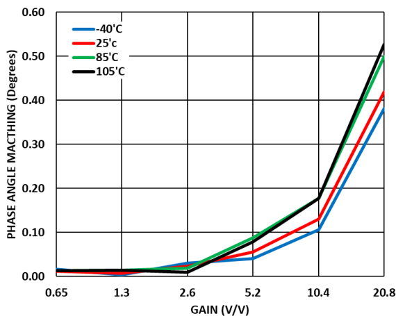
Figure 39. Phase Matching vs PGA Gain over Temperature, Normalized to Gain = 0.325 V/V
