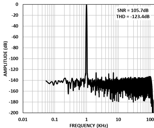
Figure 14. FFT Wideband Low Ripple FIR Filter, Differential Input, -0.5dBFS, Gain = 0.325 V/V, FDA = Full Power.
