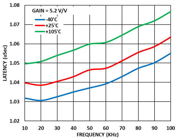
Figure 45. Analog Front End (AFE) Latency vs Frequency across Temperature, Gain = 5.2 V/V
