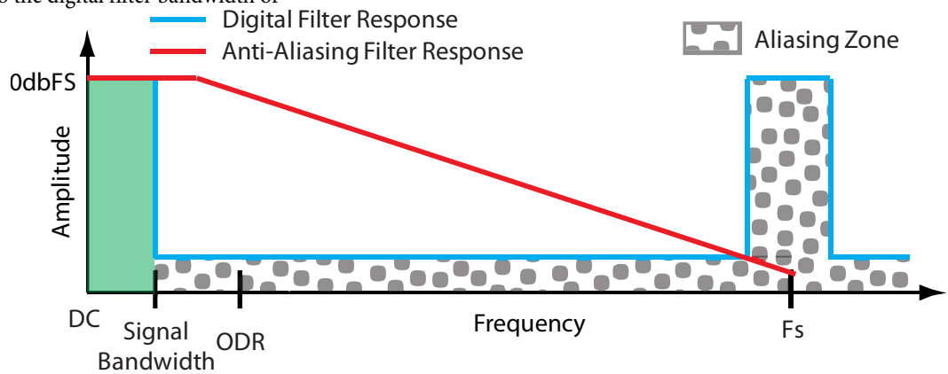
Figure 66. Simplified illustration of the overall frequency response
