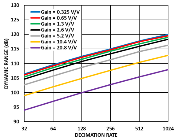
Figure 38. Dynamic Range vs Decimation Rate at Various Gain, Wideband Low Ripple FIR Filter, Shorted Input
