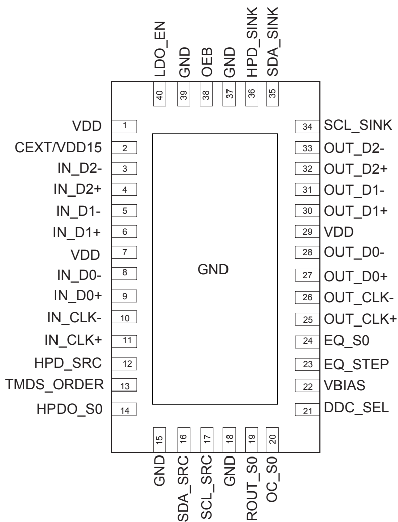
Figure 3-1 Pinout Configuration
