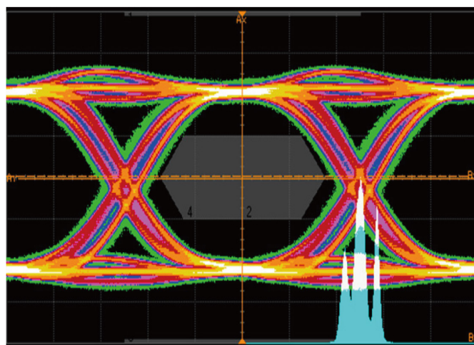
24" Input (-15.46dB loss) , EQ=2.5dB, 500mV Swing, Pre-emp =1.5dB, Rout_S0=1
