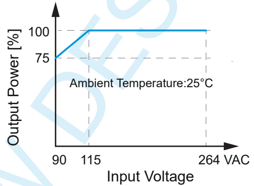
Figure 2. Input Voltage Derating Curve
