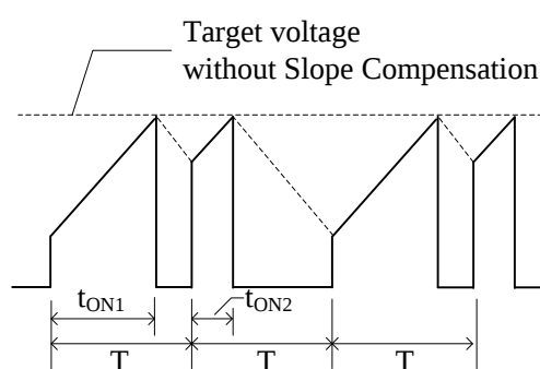
Figure 9-9 Drain current, I_D , waveform in subharmonic oscillation
