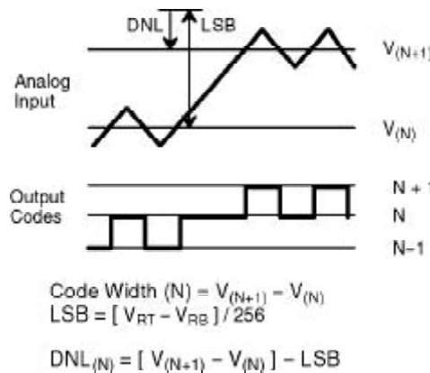
Figure 2. DNL Measurement
