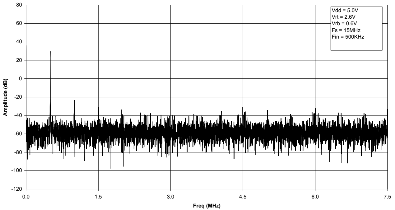
Graph 10. FFT Plot
