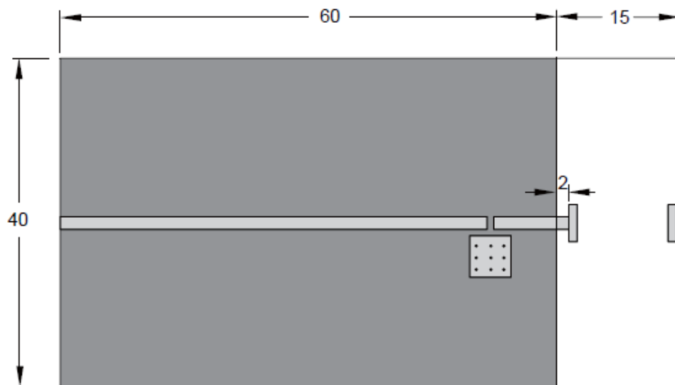
Fig. 2 Outlook and dimension of evaluation board
