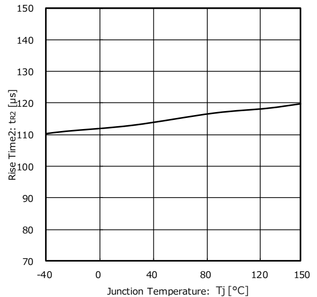
Figure 20. Rise Time2 vs Junction Temperature (RSR = 68 kΩ)
