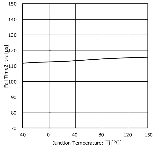
Figure 18. Output Fall Time2 vs Junction Temperature (RSR = 68 kΩ)
