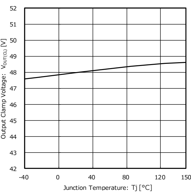
Figure 12. Output Clamp Voltage vs Junction Temperature
