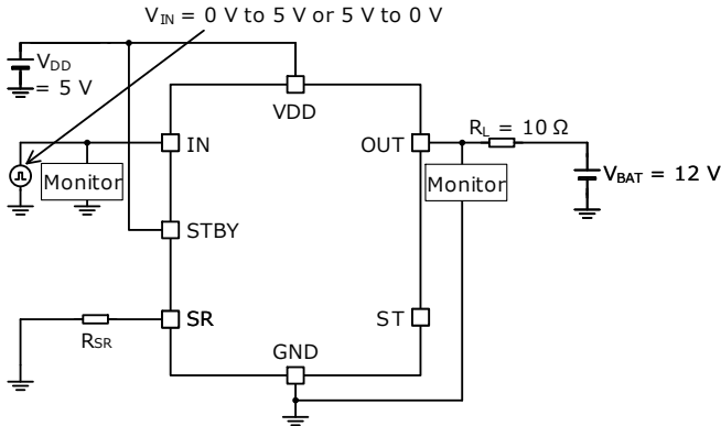
Measurement Circuit for Figure 13, Figure 14, Figure 15, Figure 16, Figure 17, Figure 18, Figure 19, Figure 20, Figure 21, Figure 22, Figure 23 and Figure 24
