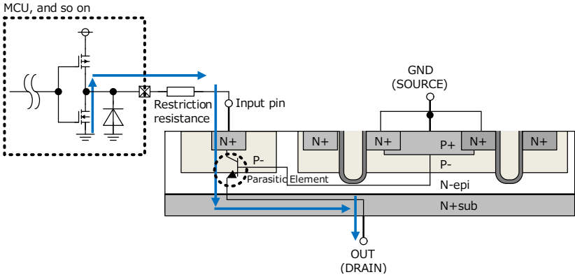
Figure 35. Negative Current Path (when the input pins are Low)
