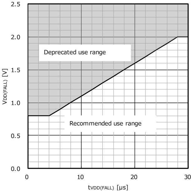
Figure 37. Recommended Use Range
