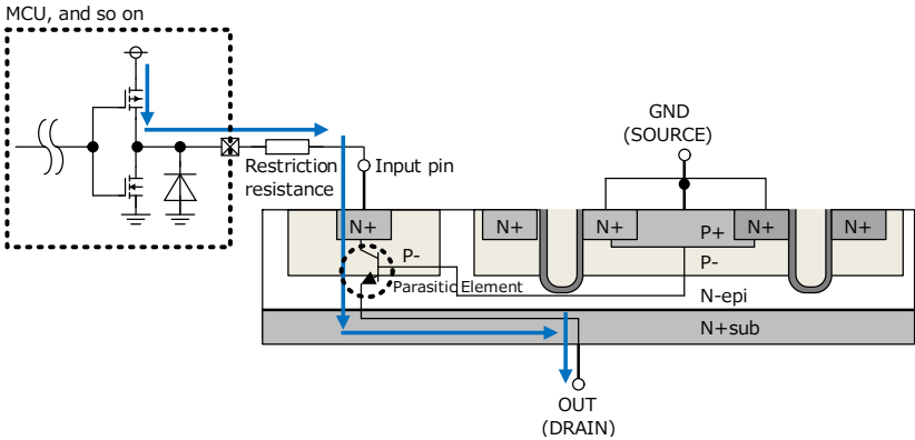
Figure 33. Negative Current Path (when the input pins are High)
