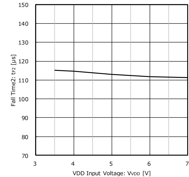
Figure 17. Output Fall Time2 vs VDD Input Voltage (RSR = 68 kΩ)
