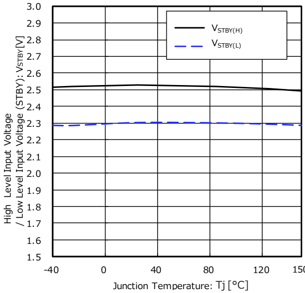
Figure 4. High Level Input Voltage / Low Level Input Voltage (STBY) vs Junction Temperature
