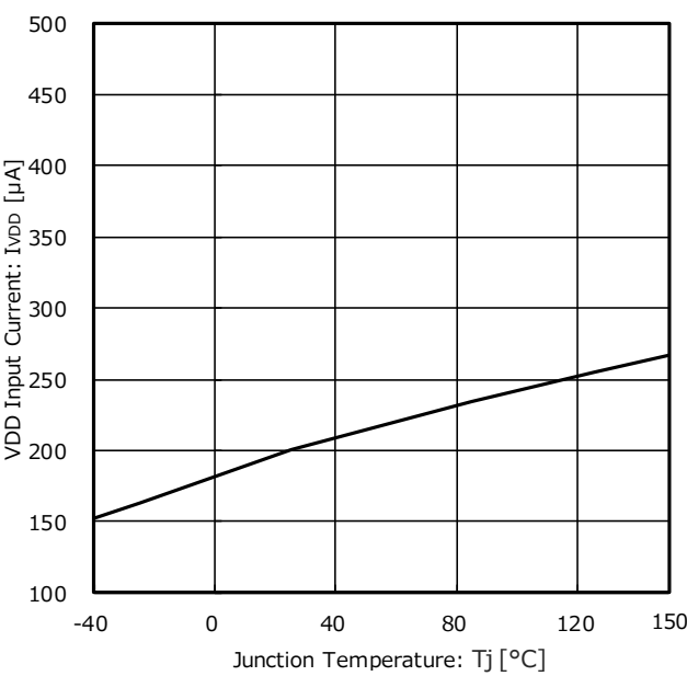
Figure 2. Operating Current vs Junction Temperature
