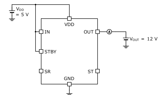
Measurement Circuit for Figure 25
