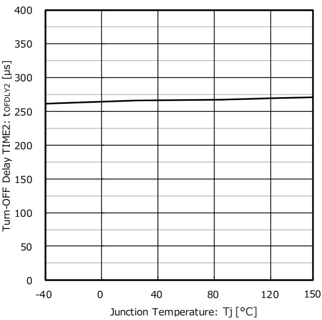
Figure 16. Turn-OFF Delay Time2 vs Junction Temperature ( R_{SR} = 68\text{ k}\Omega )
