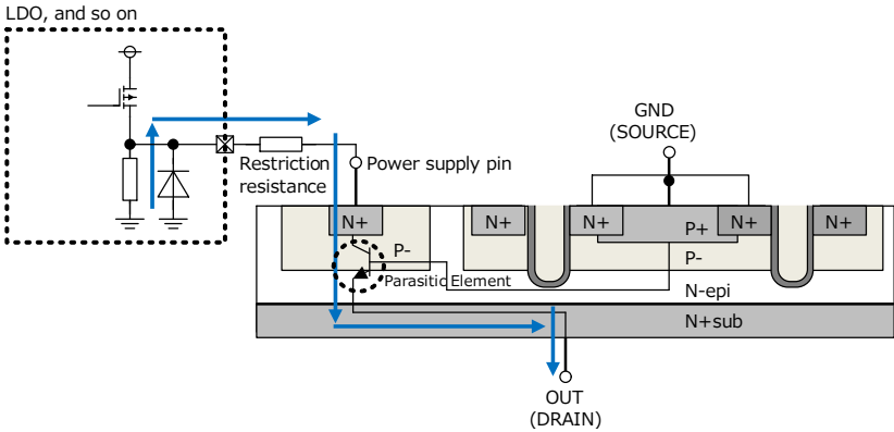
Figure 34. Negative Current Path (when the power supply pin is Low)
