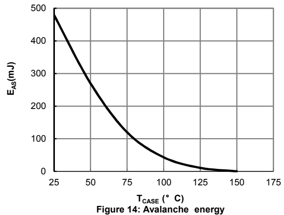
Figure 14: Avalanche energy
