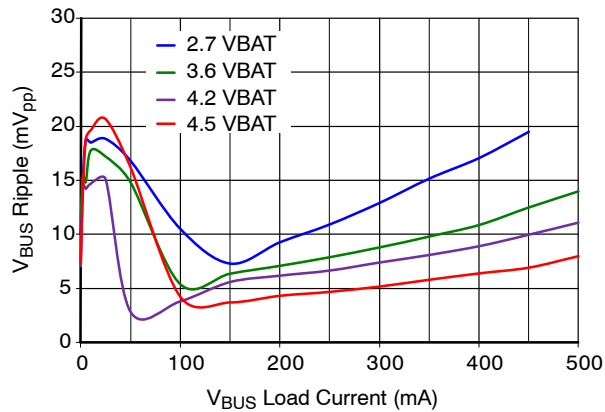
Figure 25. Output Ripple vs. V_{BAT}
