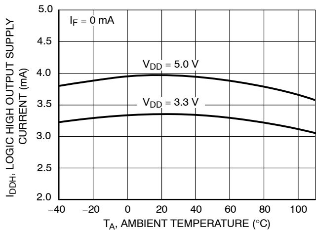
Figure 5. Logic High Output Supply Current vs. Ambient Temperature
