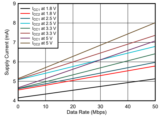
Figure 5-10. ISO6763-Q1 Supply Current vs Data Rate (With No Load)
