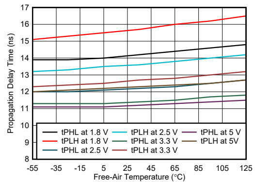
Figure 5-12. Propagation Delay Time vs Free-Air Temperature
