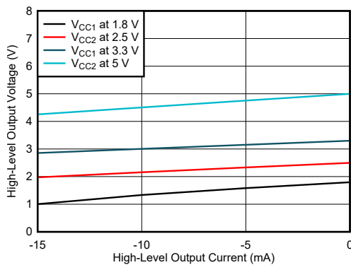
Figure 5-11. High-Level Output Voltage vs High-level Output Current
