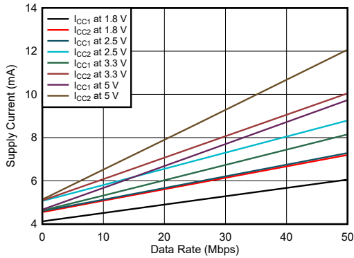
Figure 5-9. ISO6763-Q1 Supply Current vs Data Rate (With 15-pF Load)
