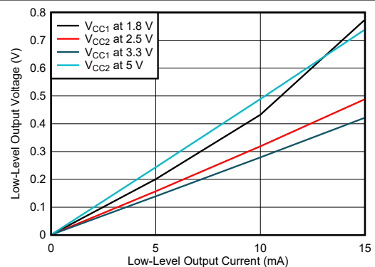
Figure 5-14. Low-Level Output Voltage vs Low-Level Output Current
