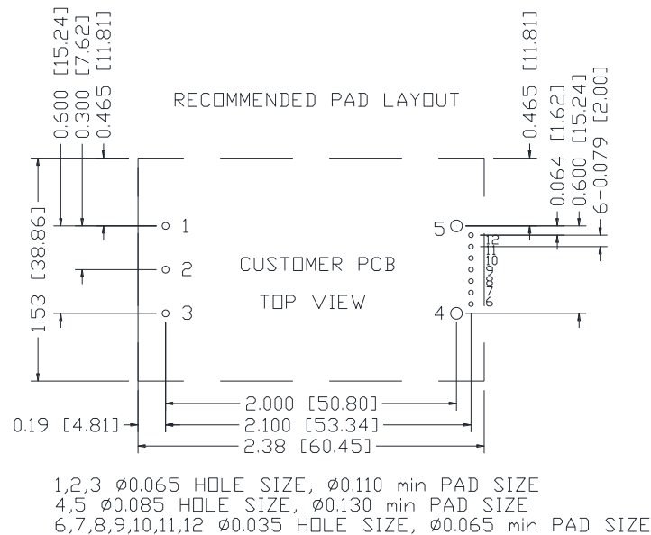
Figure 36. Recommended pad layout
