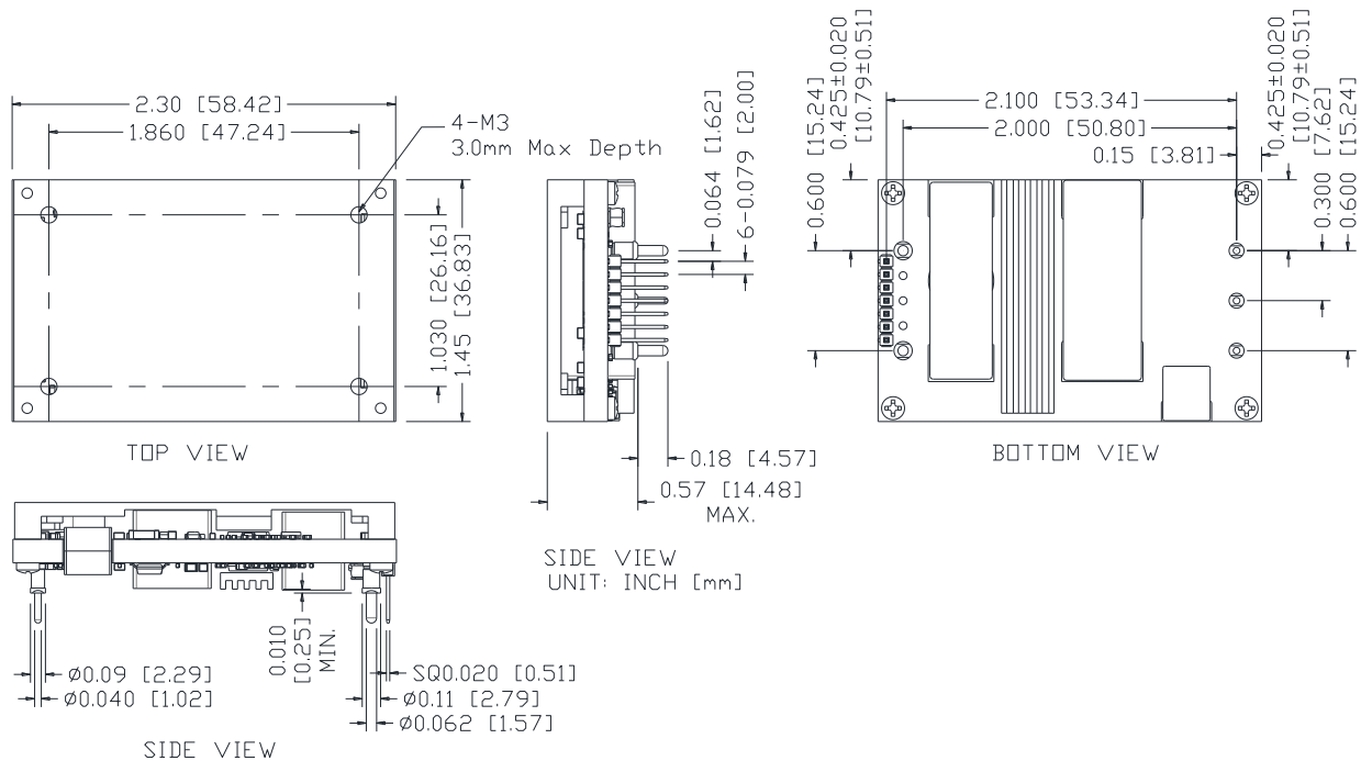
Figure 32. 0RQP-E0S12A/B/P Outline
