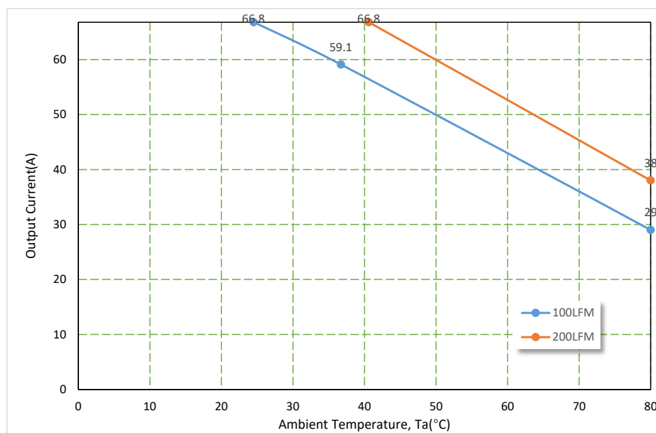
Figure 26. Thermal derating curve 0RQP-E0S12C Airflow from V_O to V_{IN}
