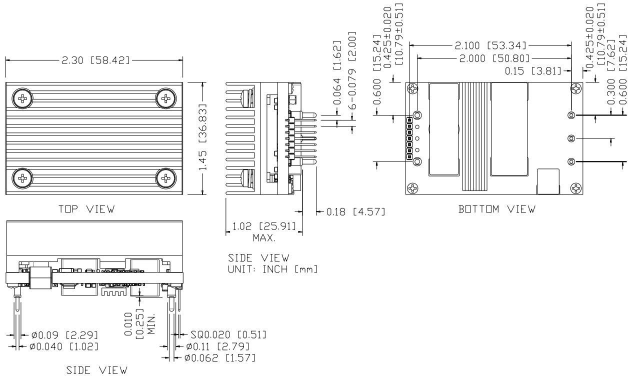
Figure 33. 0RQP-E0S12C Outline
