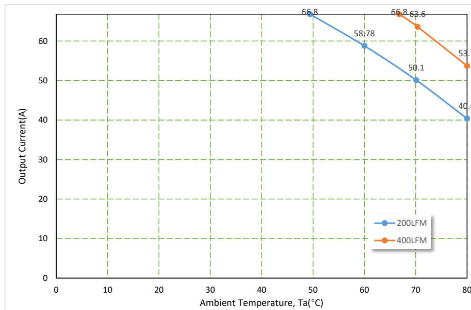
Figure 25. Thermal derating curve – with external Heatsink 0RQP-E0S12A/B/P/BN Airflow from V_O to V_{IN}
