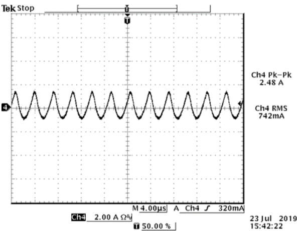
Figure 12. ic (input terminal ripple current), AC component
