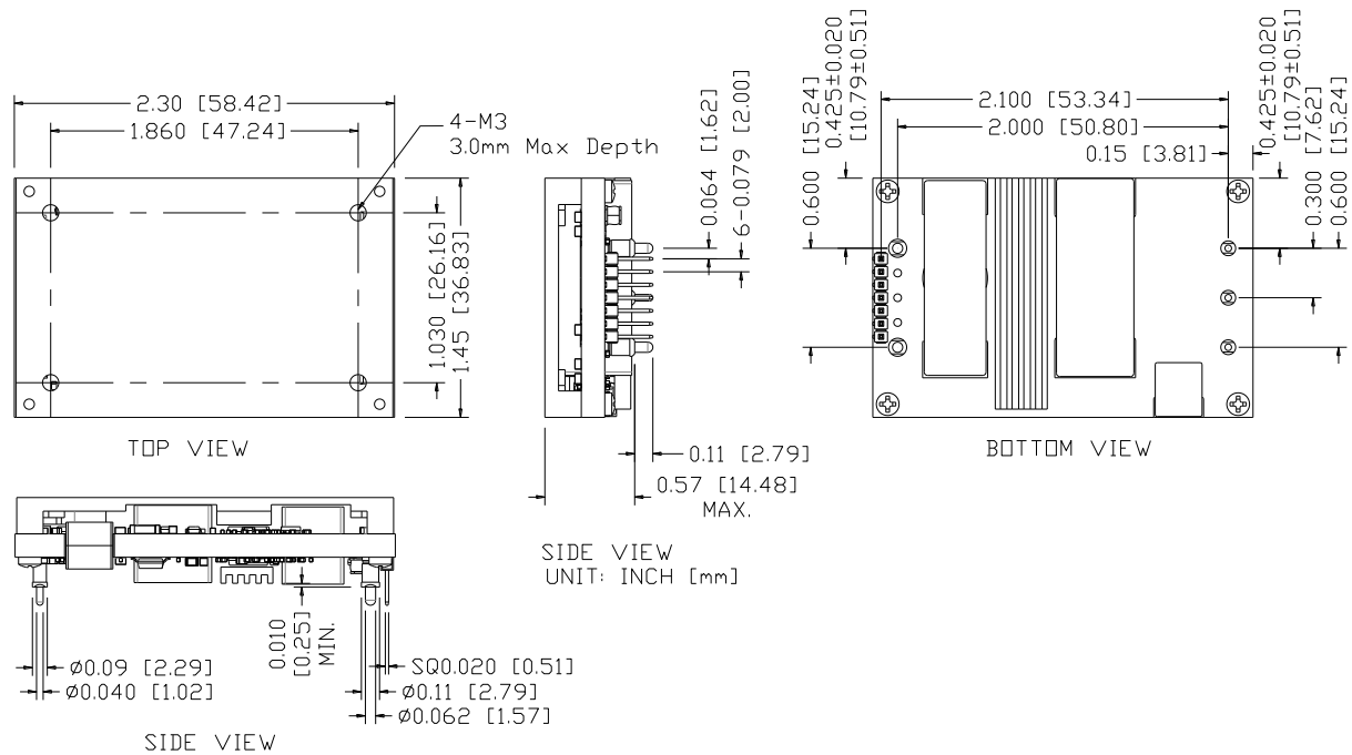
Figure 34. 0RQP-E0S12BN Outline
