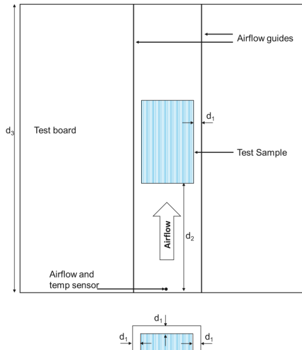
Figure 24. Thermal test setup, Airflow from V_O to V_{IN}
