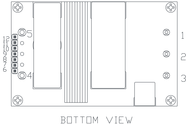
Figure 35. Pins
