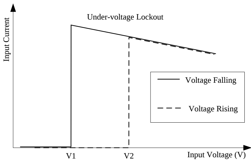
Figure 27. Under voltage lockout V_1 = 36.5\text{ V} V_2 = 38.5\text{ V}
