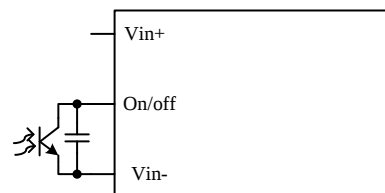
Figure 3. Control with photocoupler circuit
